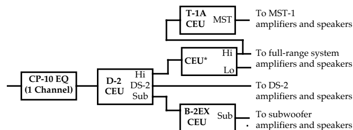
Five-way system flow block.
