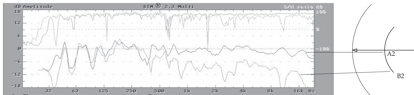
Fig 3.3d Comparison of on-axis near (A2) and off-axis near (B1).
