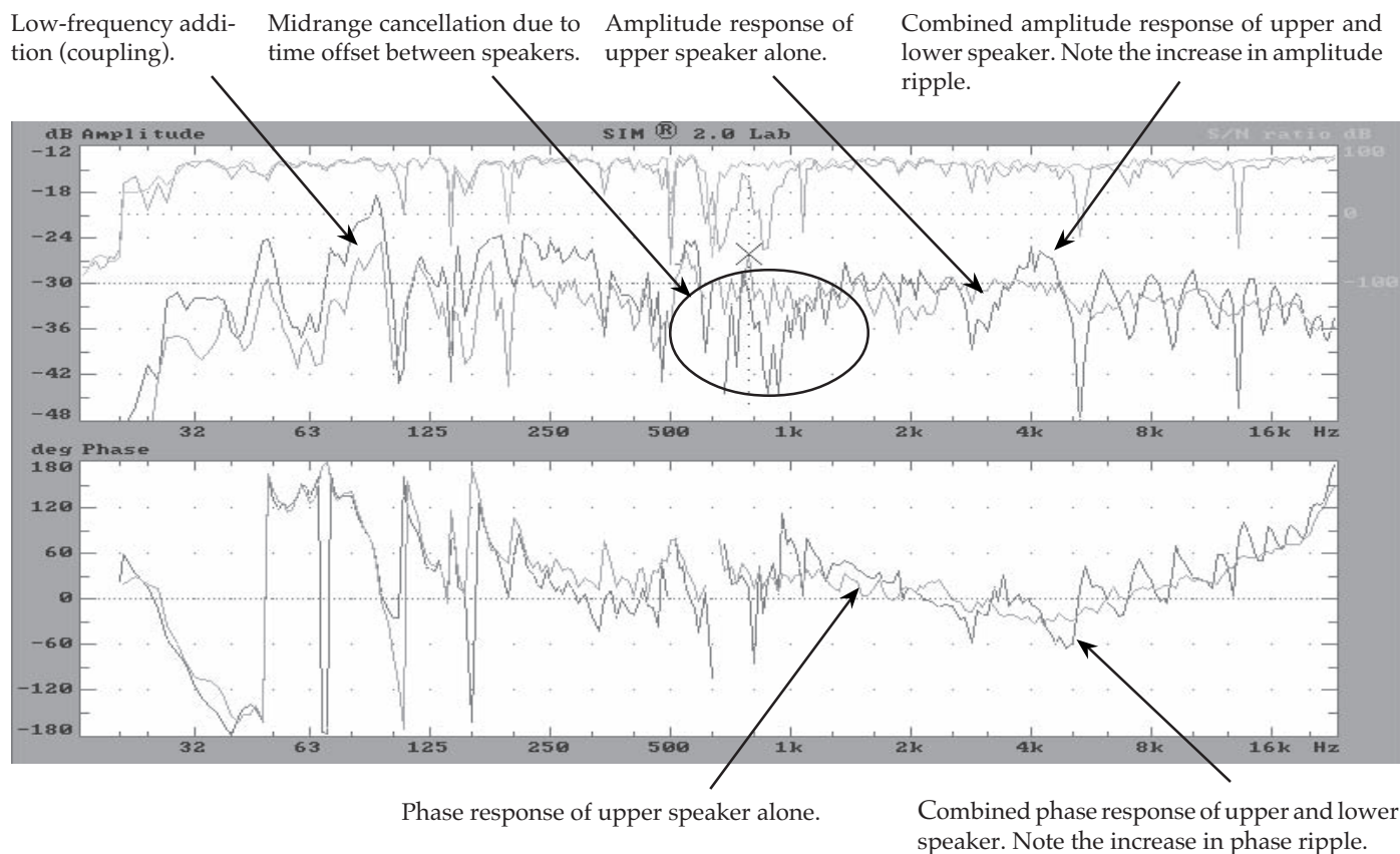
Fig 2.2d Comparison frequency response of single speaker to combination.
