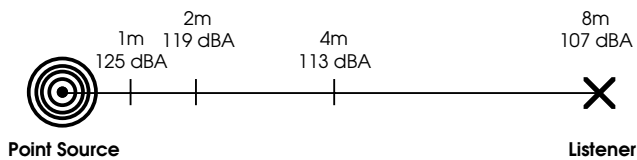
Fig 3.3a Inverse square law propagation loss.
