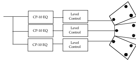
Excess System Subdivision
