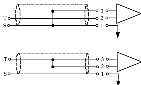
Fig 4.8e Unbalanced cable with mono phone jack.
