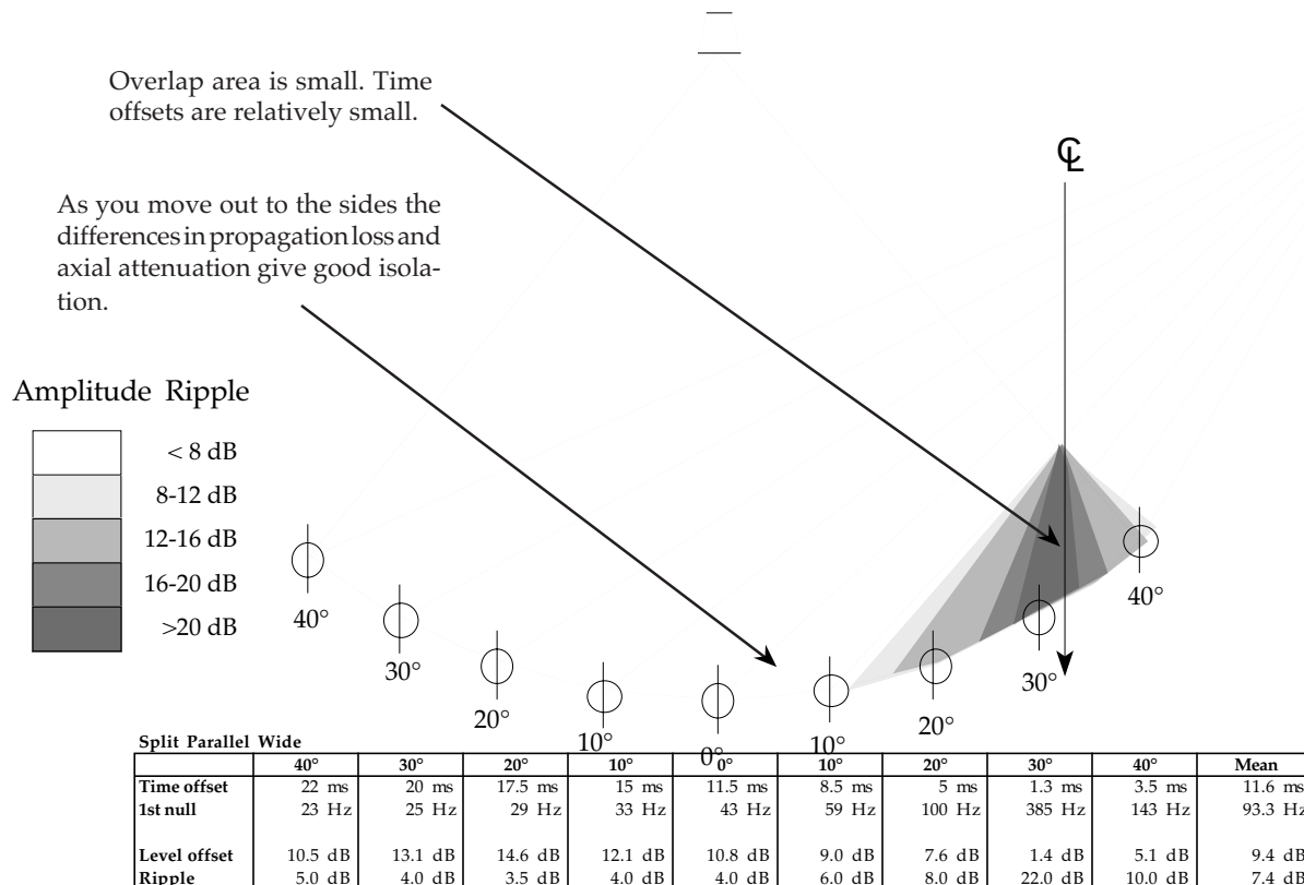
Fig 2.2x Split-parallel (wide) array interaction.
