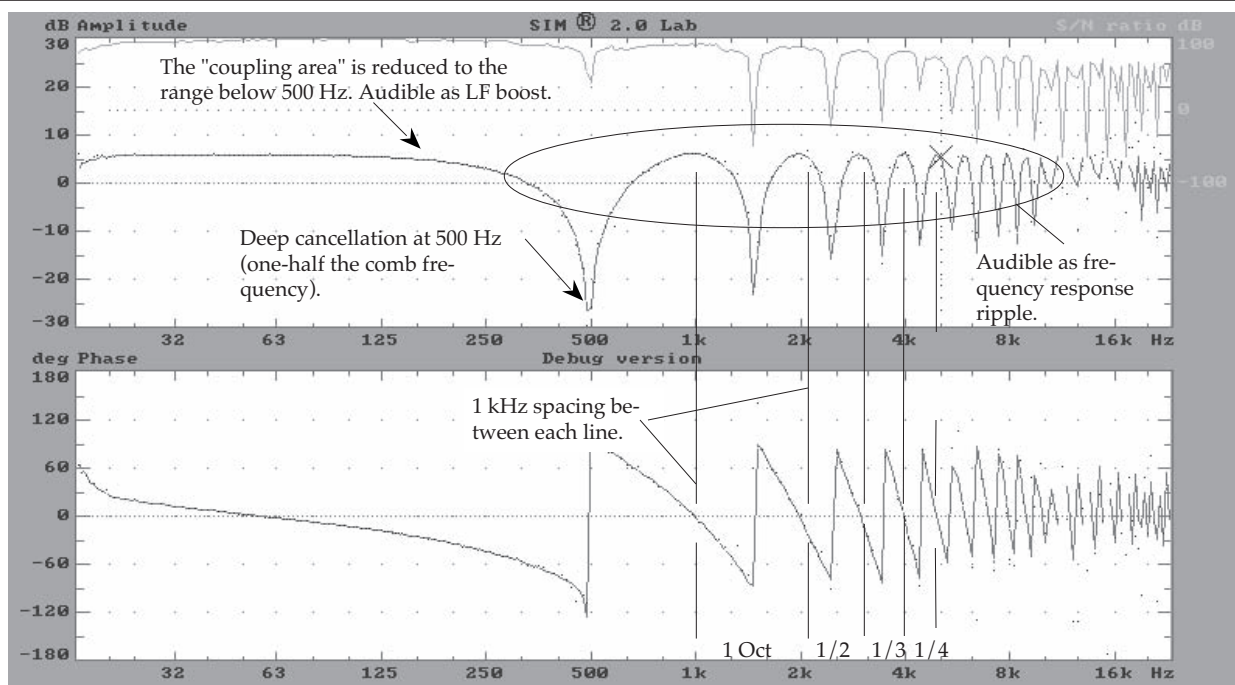
Fig 2.1f Comb filtering with 1 ms time offset between signals with 0 dB level offset.
