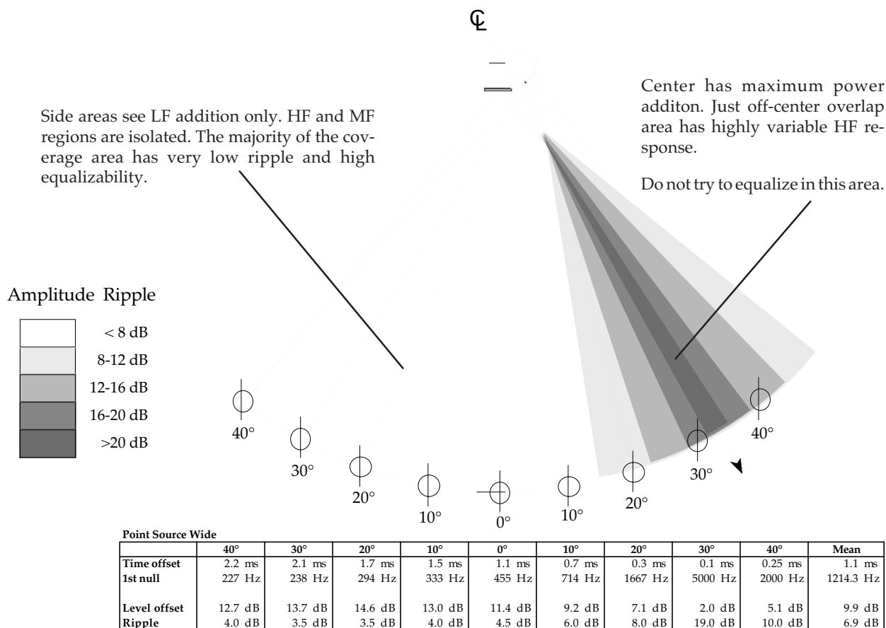
Fig 2.2q Wide Point-Source Array Interaction.
