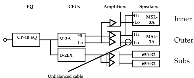
Fig 4.8i Flow block diagram of the system. The cable driving the left outer LF channel was unbalanced, creating the frequency response problems shown in Fig 4.8h below.
