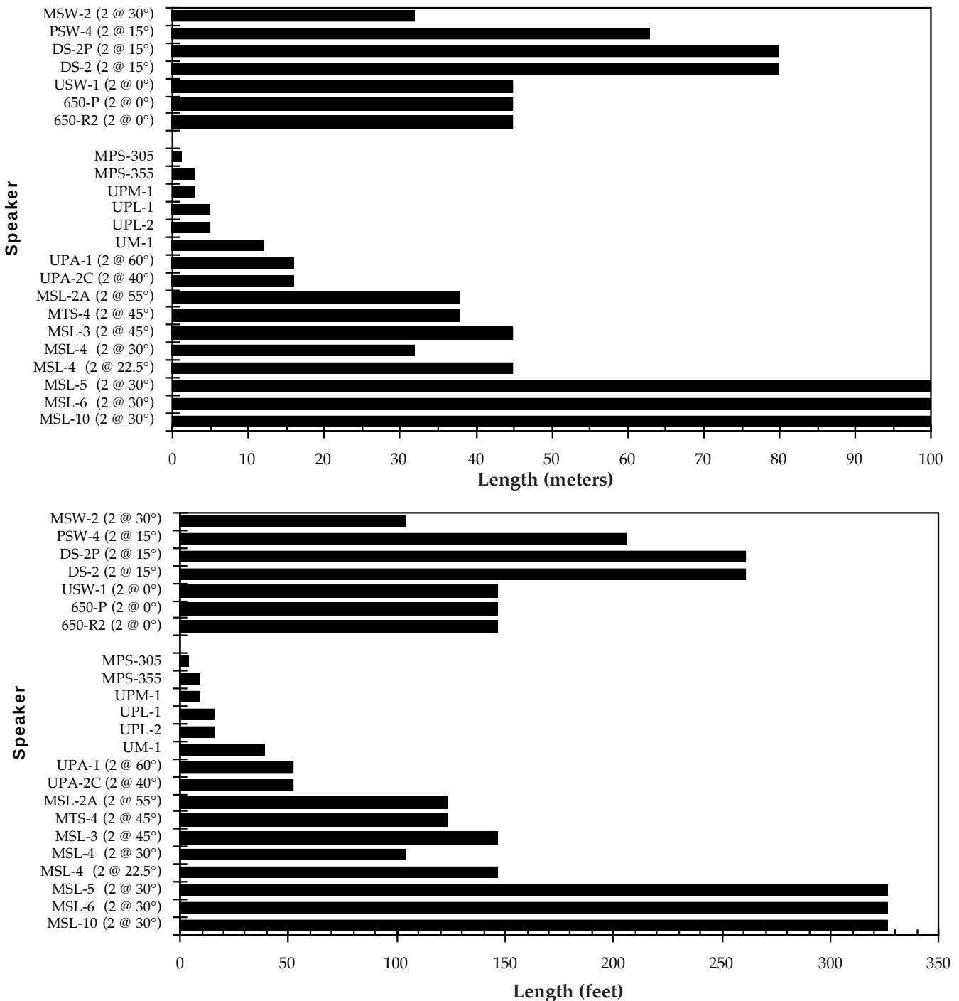
Fig 3.3c Meyer speaker SPL/distance reference (meters and feet).
