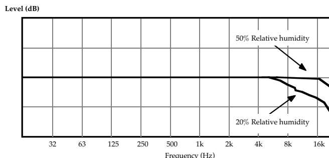
Fig 2.4b Relative humidity effect on frequency response.
