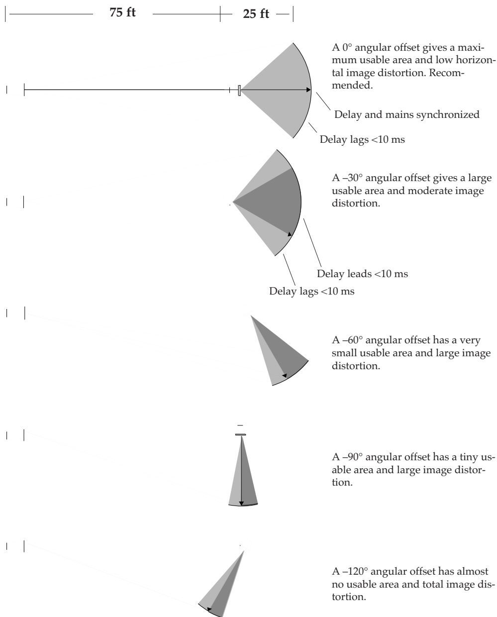
Fig 3.7n Usable horizontal angle for distributed delays.
