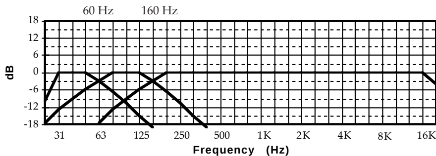
Four-way system frequency range chart.
