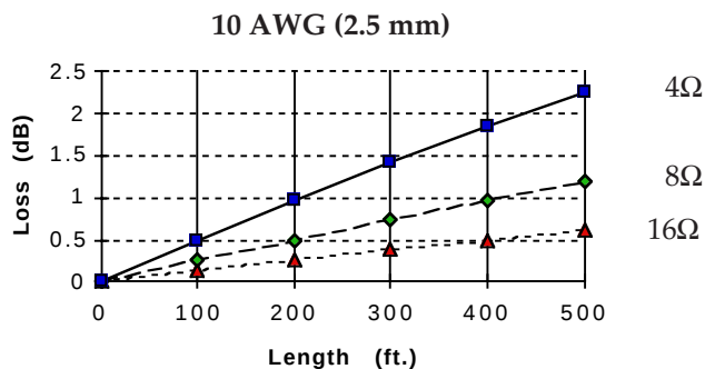
Fig. 1.7.k Cable loss over distance for 10 AWG (2.5 mm).
