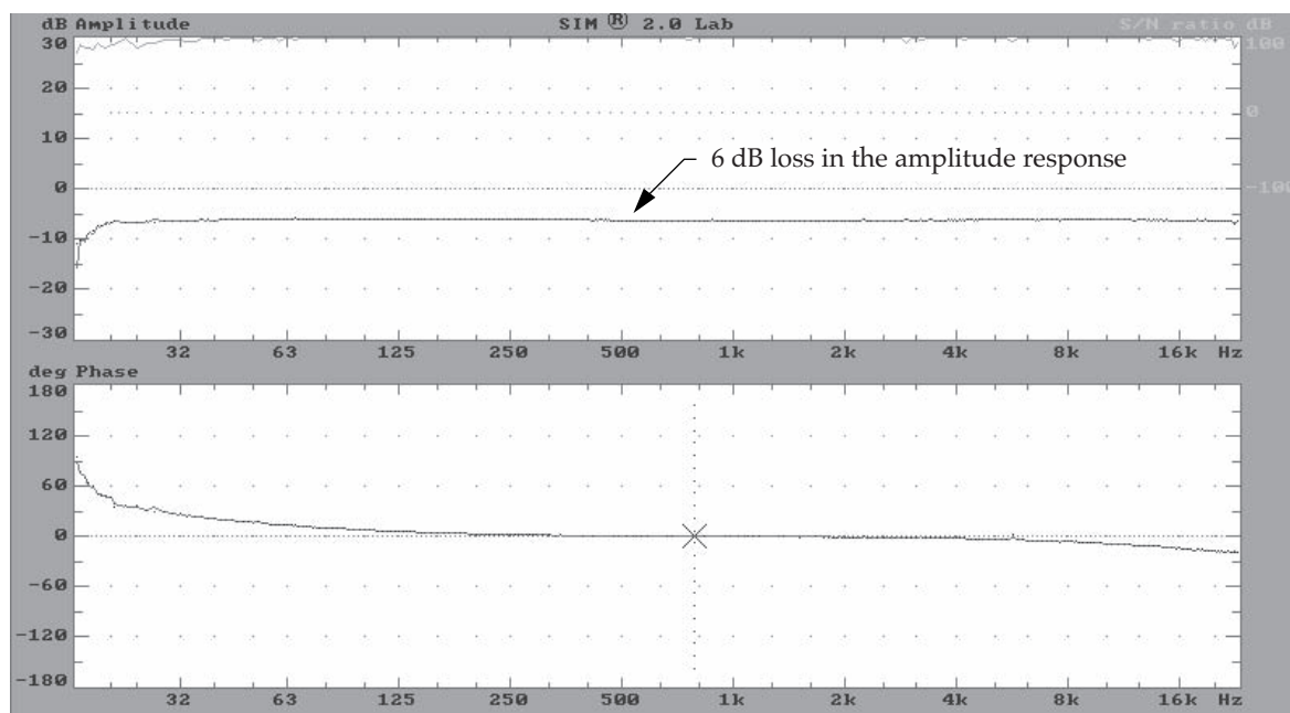
Fig 4.8g Frequency response of a balanced line that has become unbalanced. The amplitude response shows a broadband 6 dB loss due to the loss of one-half of the voltage drive. The phase response is unchanged from the balanced scenario
