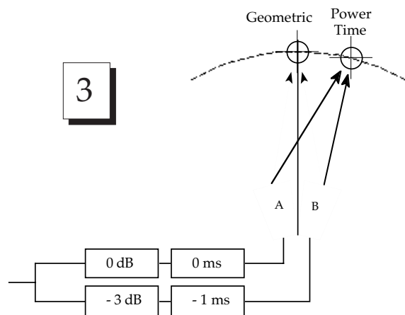
Fig 5.7i Delay tapering—Time center moved to power center.
