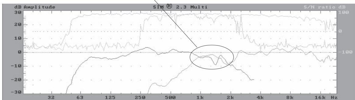
Fig 1.4h UPA-1C with matched voltage gains at crossover.
