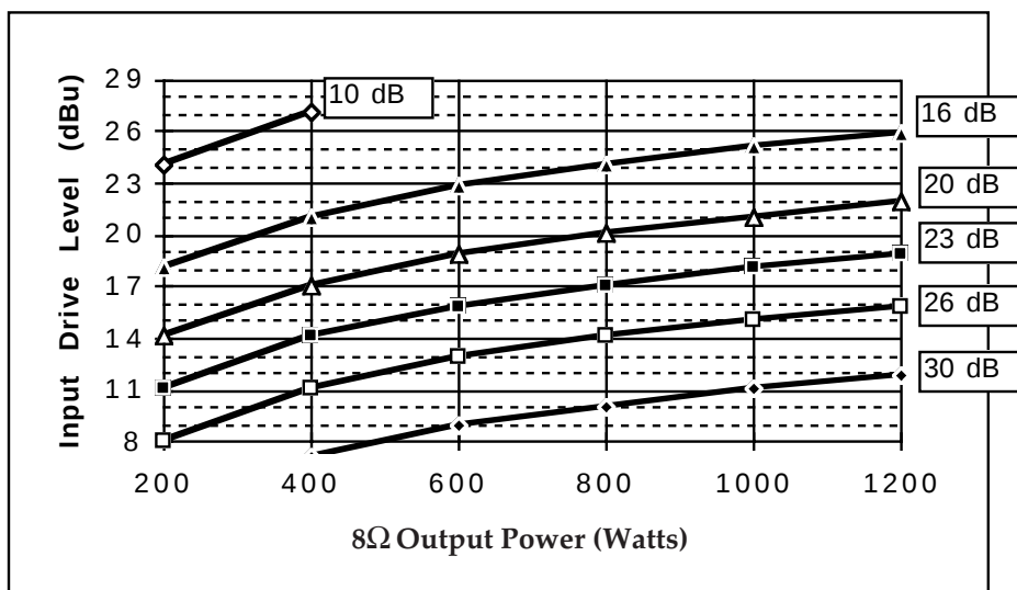
Fig 1.4f Drive level requirements for full power amplifier output.
