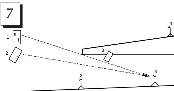
Lobe study analysis of the main cluster into the underbalcony area.
