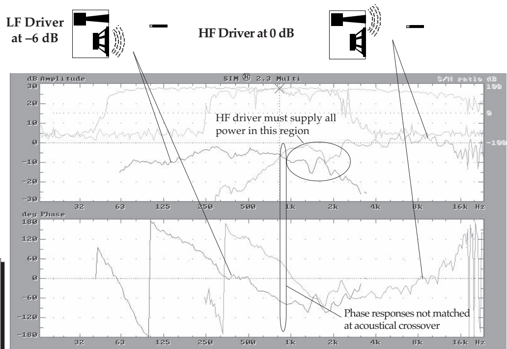
Fig 4.10b Misaligned crossover of the UPA-1C. The LF amplifier was set to -6 dB.
