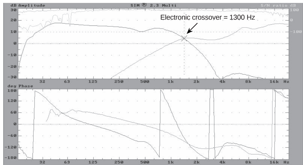
Fig 1.2a Electrical response of S-1 CEU.
