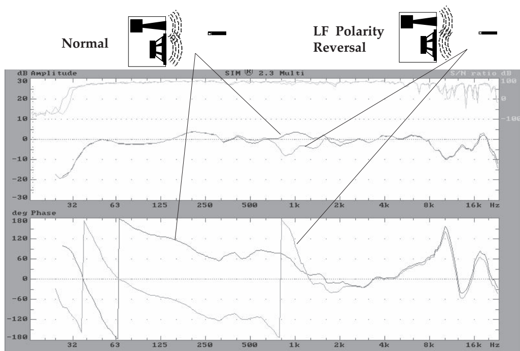
Fig 4.9g Polarity reversal of LF driver compared to a normal system.
