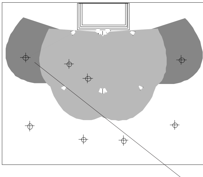
Plan view of the hall indicating the mic position and speaker status during the measurements shown opposite.
