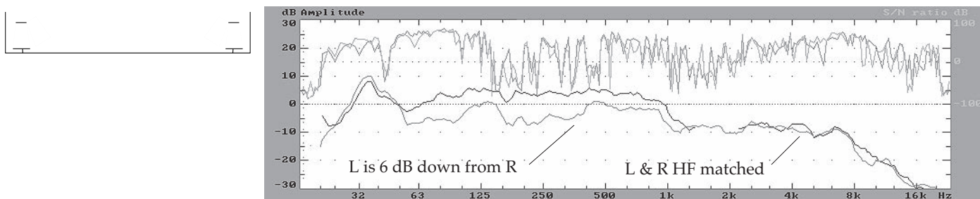
C. Outer speakers only. The midrange area shows a 6 dB difference in level. This was caused by an unbalanced cable driving the amplifier.
