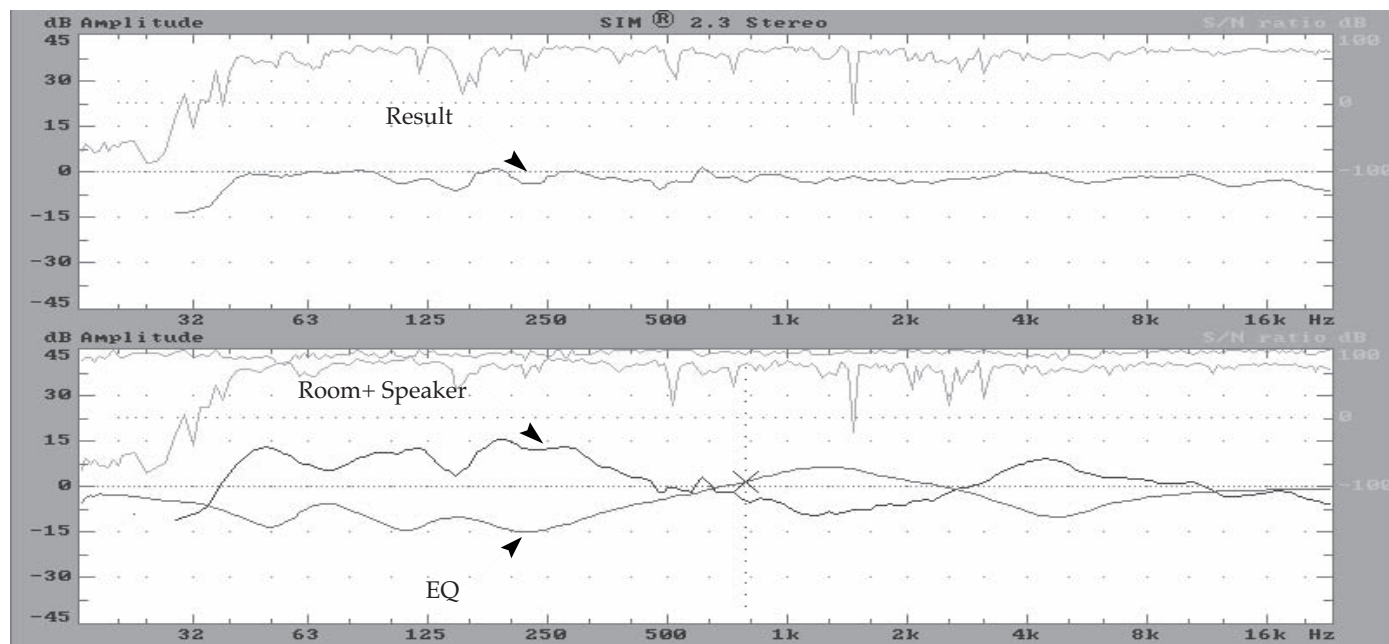
Fig 5.8b Group view of the three SIM transfer functions. The equalizer response is adjusted until it has created an inverse of the room+speaker response. This creates a flat response in the result.
