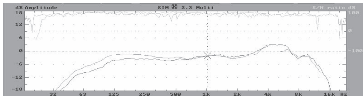
Fig 1.9b Frequency response of the industry standard vocal microphone, complete with proximity effect, presence peak and 20 dB loss at 16 kHz. Note the amplitude scale is 6 dB/division in contrast to the 2 dB/division of the above screen (Fig 1.9a).
