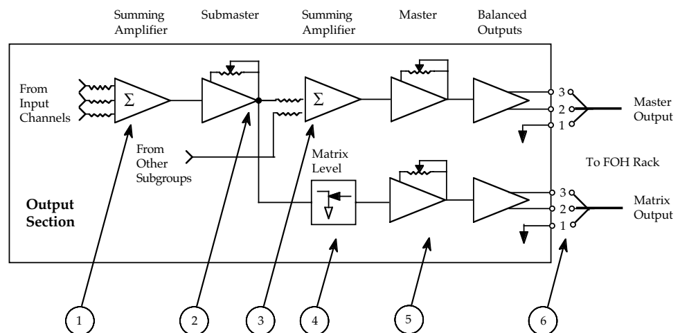
Fig 4.4b Output section verification.
