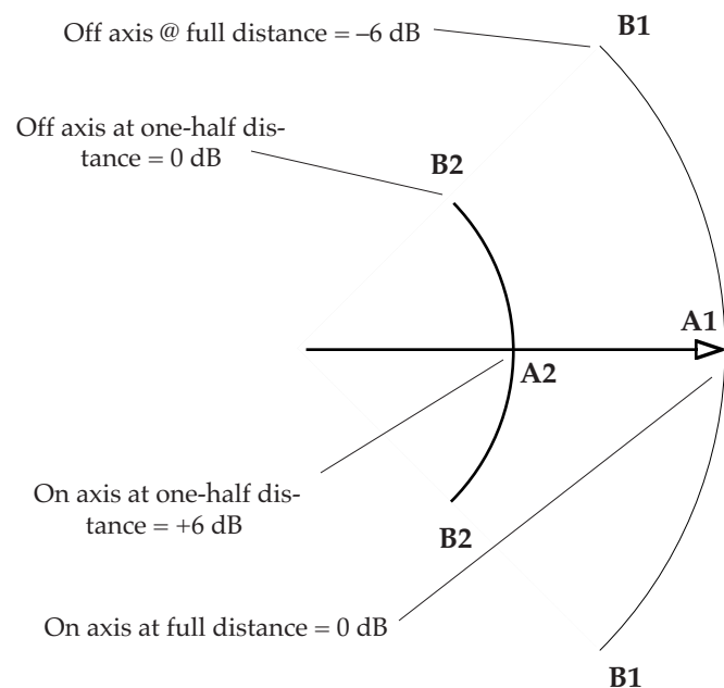
Fig 3.3b Relationship between propagation loss and coverage pattern.
