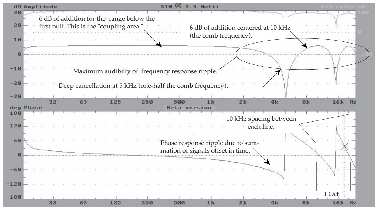
Fig 2.1e Comb filtering with .1 ms time offset between signals with 0 dB level offset.
