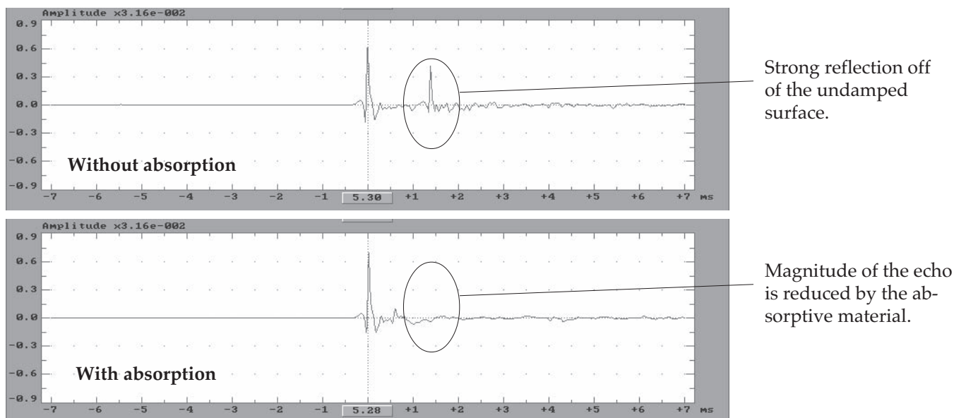
Fig 5.4a Effect of absorptive materials on the impulse response.
