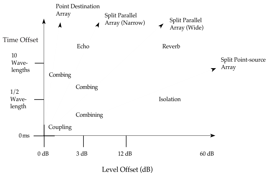
Fig 2.2g Tendencies of split speaker arrays.
