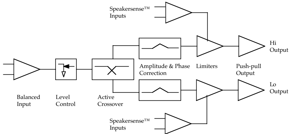
Fig 1.1a Basic flow block and connection diagram.
