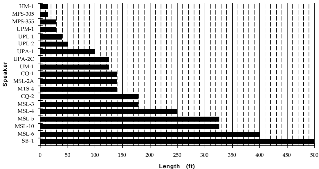
Fig 3.7l Delay speaker reference (feet).
