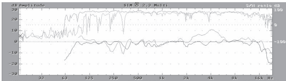
Fig 3.5e This is the amplitude response of two separate systems at their respective on-axis locations before equalization. The responses are not matched in the 4 kHz range. Therefore, separate equalization should be applied.
