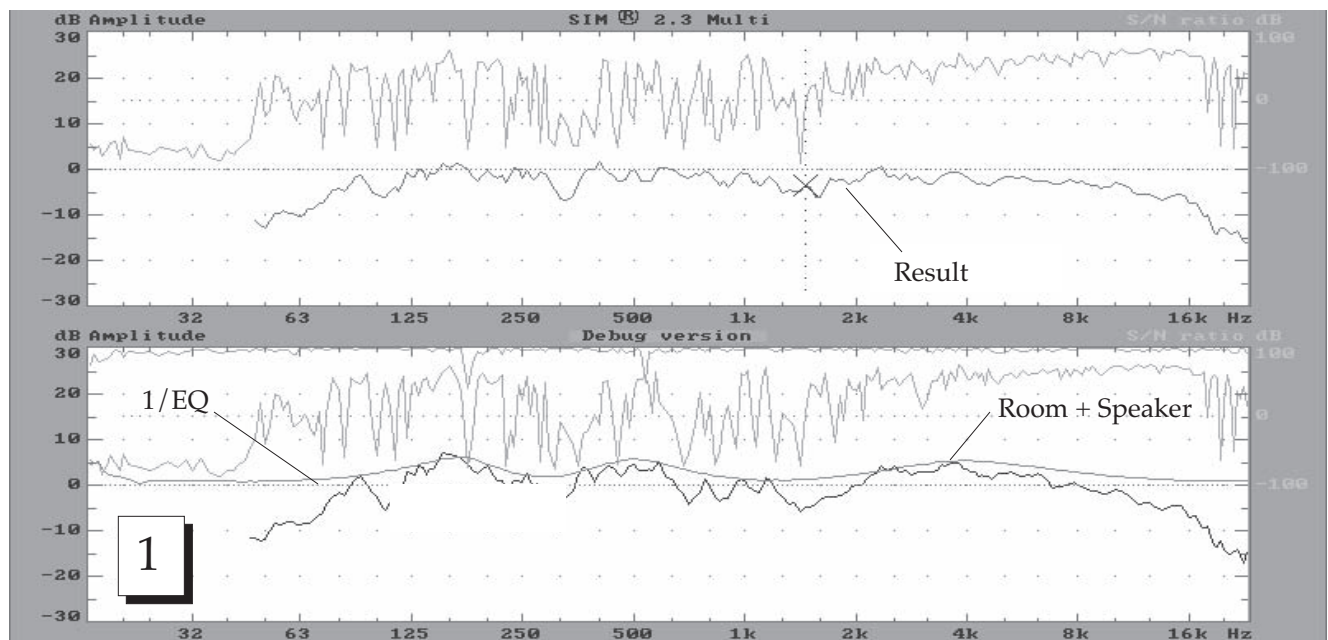
Fig 5.9a Single system analysis of the underbalcony system.
