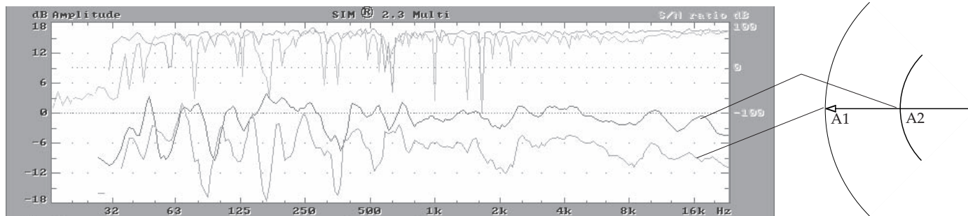
Fig 3.3c (1) Comparison of on-axis far (A1) and on-axis near (A2).
