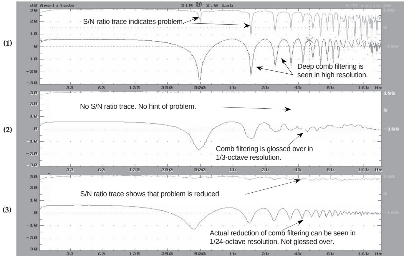
Fig 1.9d A comparison of high and low resolution for frequency response measurements.
