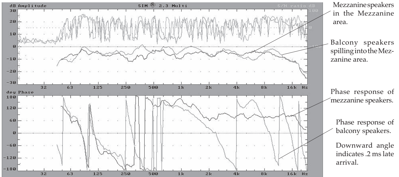
Fig 5.5c Speaker position example.
