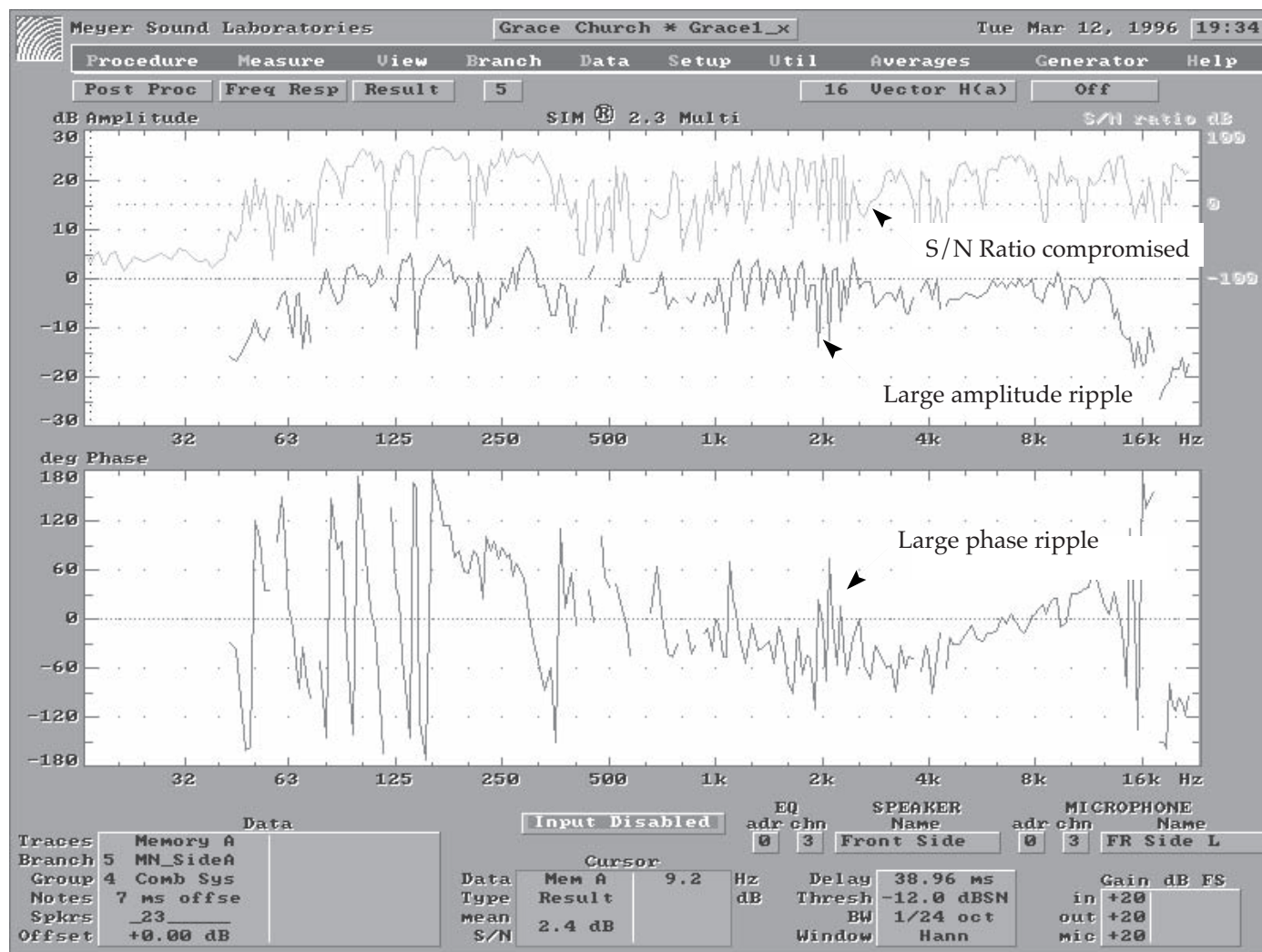
Fig 5.10j Combining the main cluster and side systems.
