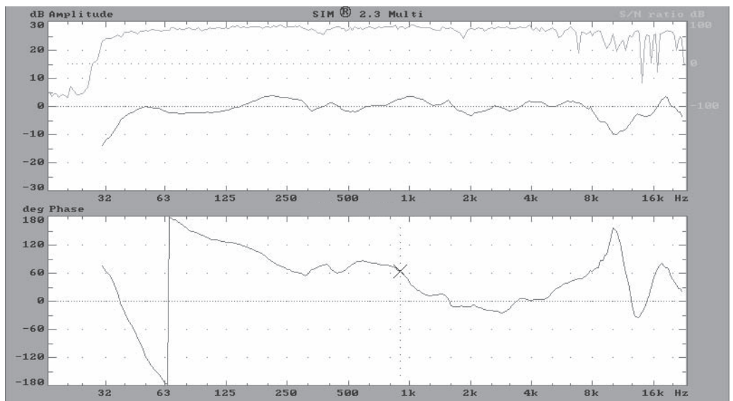
Fig 1.2c Combined acoustical response of the MSL-2A. 1
