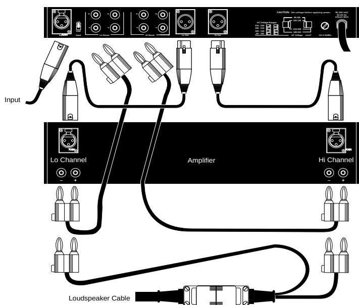
Fig. 1.3l MultiSense connection.
