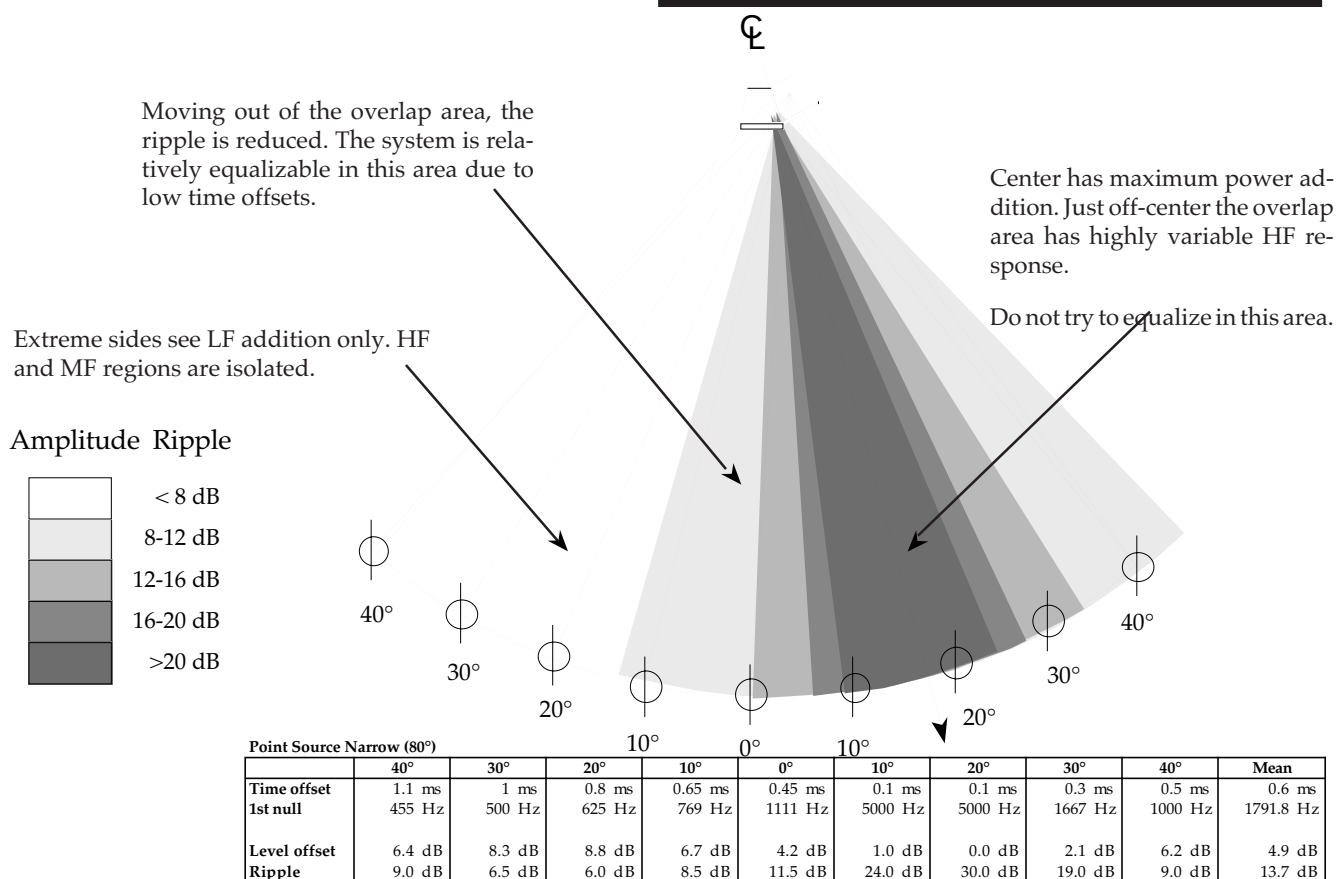
Fig 2.2j Narrow point-source array interaction.
