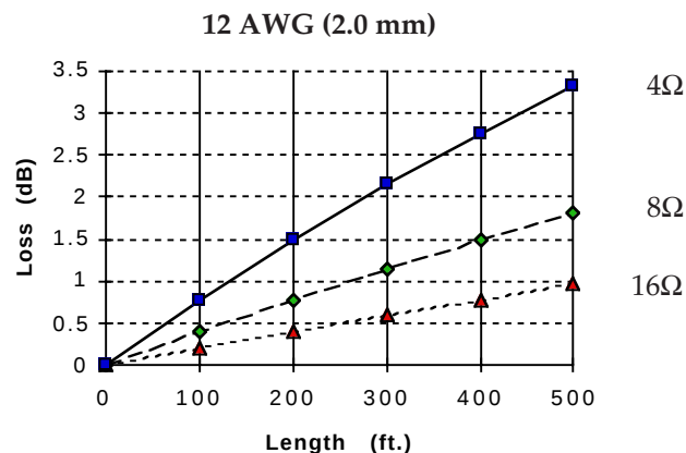
Fig. 1.7.j Cable loss over distance for 12 AWG (2.0 mm).
