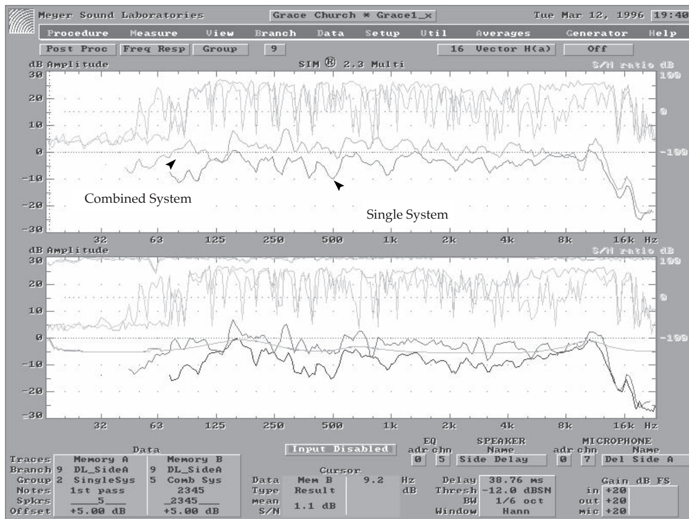
Fig 5.10n Combining the delays with the mains.
