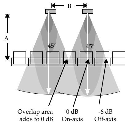
3.7j Speakers were moved closer together to optimize the response for the narrower speakers.
