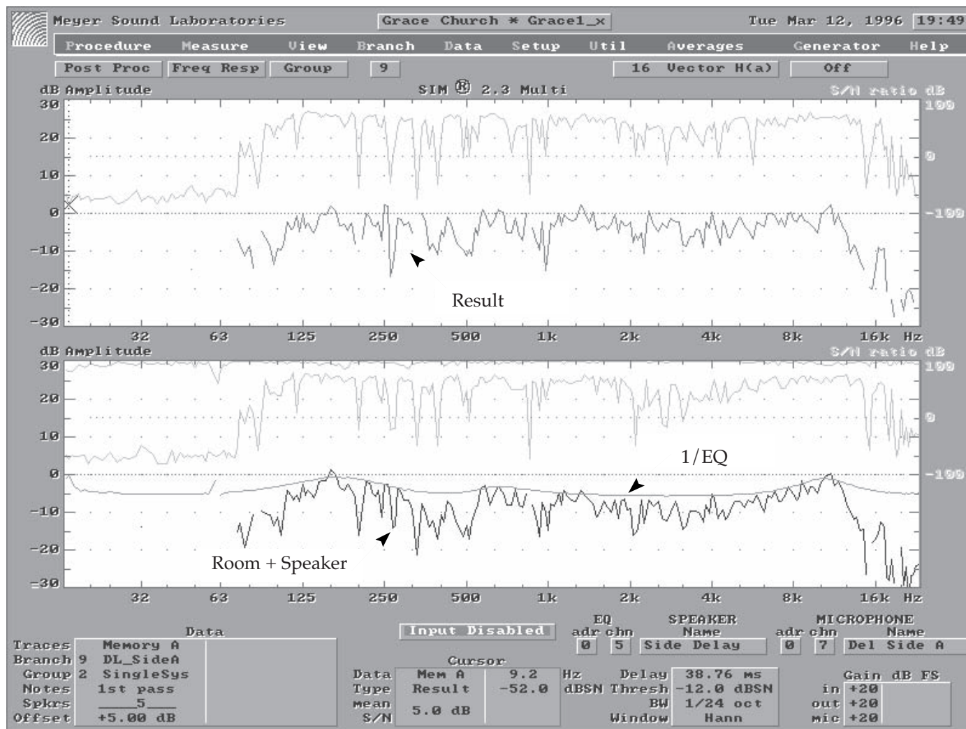
Fig 5.10I SIM equalization of the side delay speakers.
