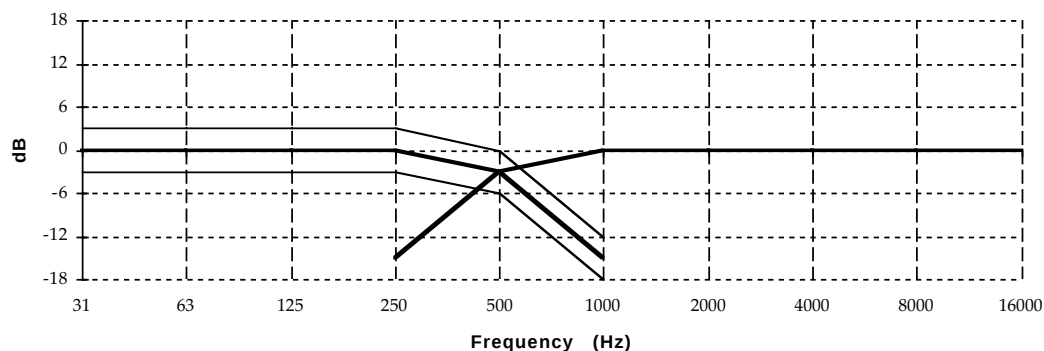
Fig. 1.4g Unbalancing the acoustic crossover.
