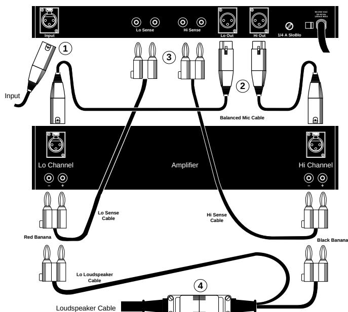
Fig. 1.3i Basic connections.
