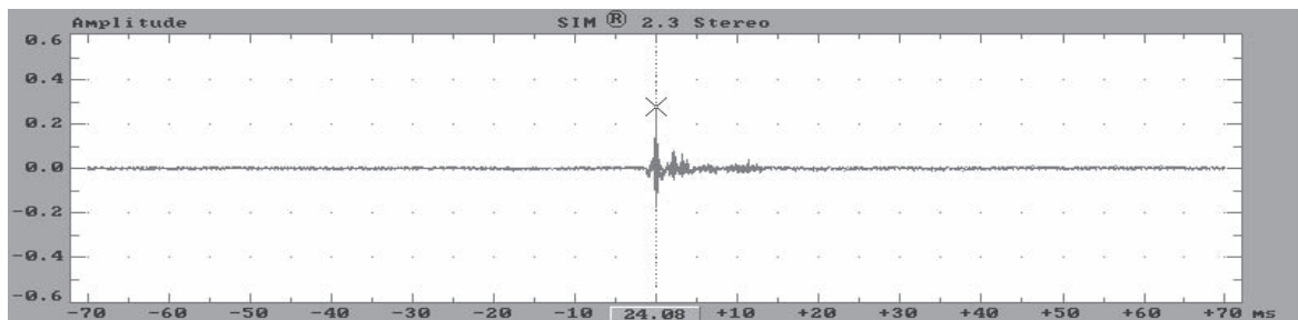
Fig 5.7f Delayfinder data indicates that the correct delay has now been added, thereby centering the impulse response.
