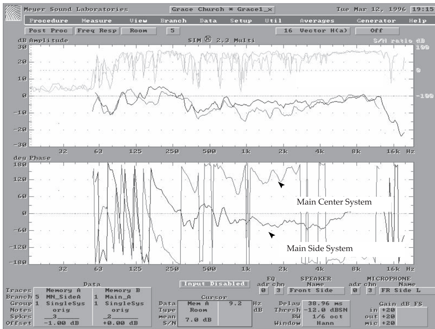
Fig 5.10g Polarity reversal discovered.
