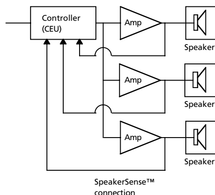
Fig. 1.3m MultiSensing one of several amplifiers. Sense lines connected to multiple CEU sense inputs.
