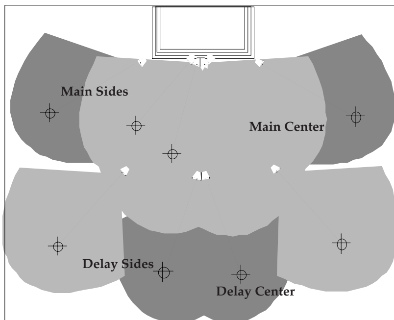
5.10a Plan view of the hall showing the intended speaker coverage zones.
