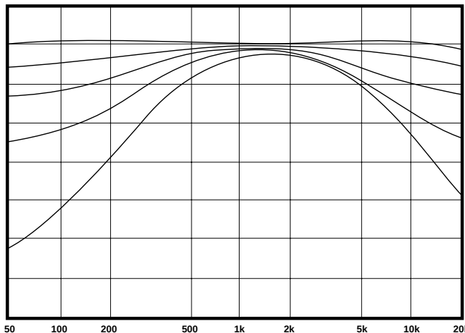
Fig 1.6b The CP-10 shelving section family of curves.
