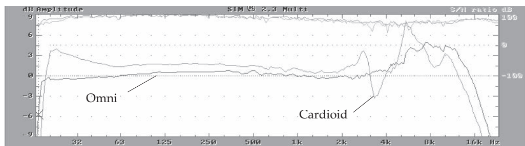
Fig 4.3e Frequency response changes with pattern switch setting.
