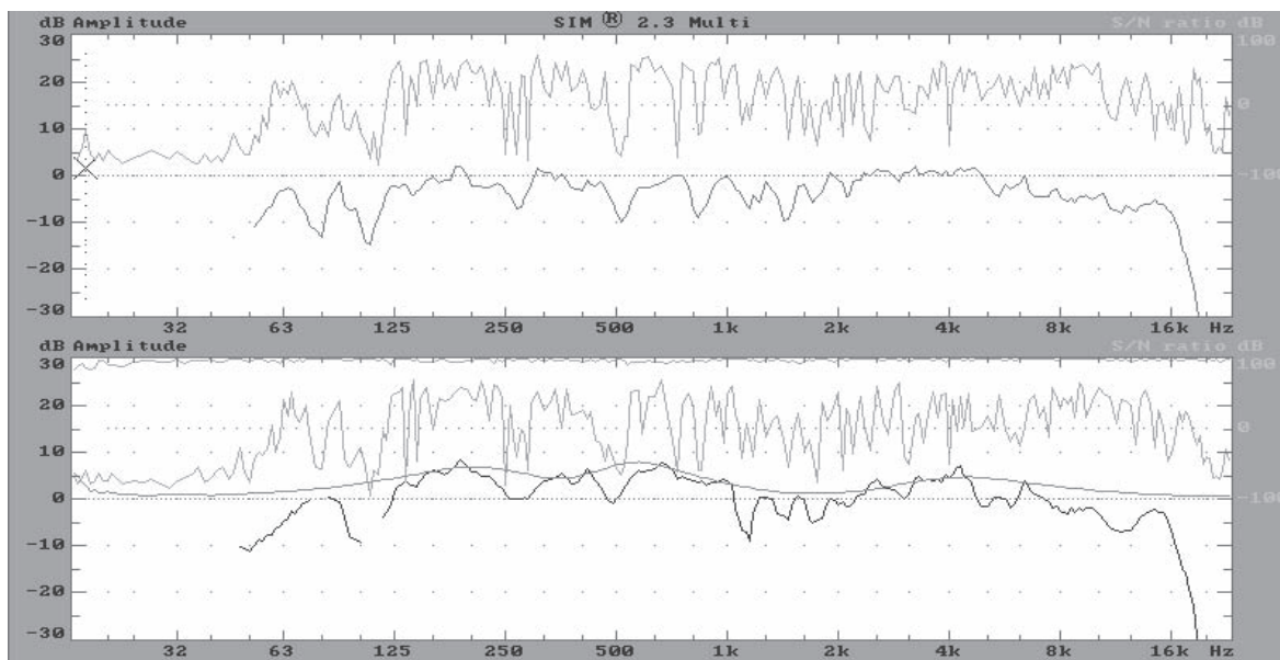
Fig 5.8f Complementary equalization example.
