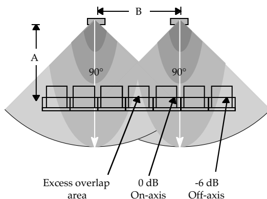
Fig 3.7h The speaker coverage angle is too wide for the current spacing. There is too much overlap, which will cause a hot spot between the two speakers.
