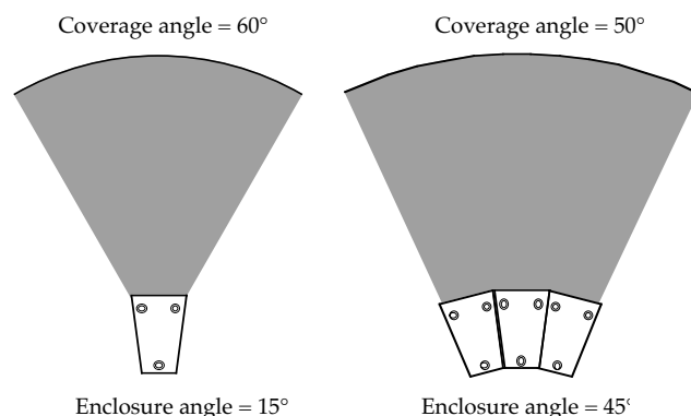
Fig 3.6d MSL-3A coverage pattern narrows while on-axis power increases as additional units are packed together. Use this configuration for long-throw applications.
