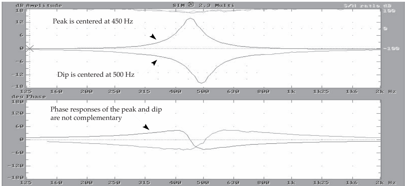
Fig 1.6h Peak and dip do not have the same center frequency.
