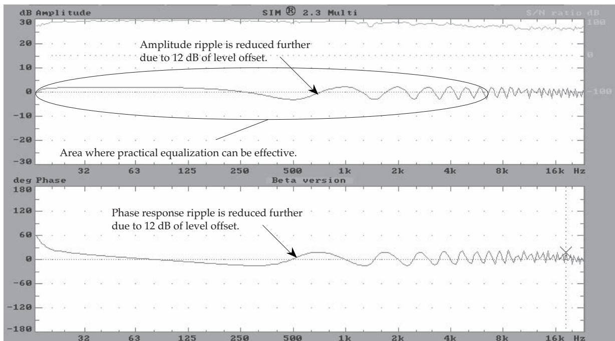
Fig 2.1j Comb filtering with 1 ms time offset between signals with 12 dB level offset.
