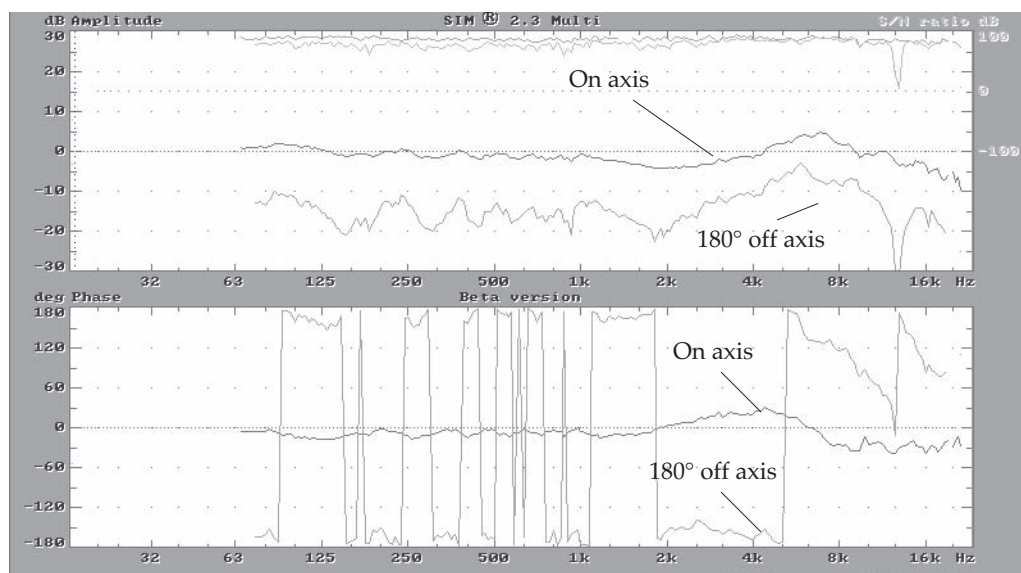
Fig 4.3f Microphone pattern verification.
