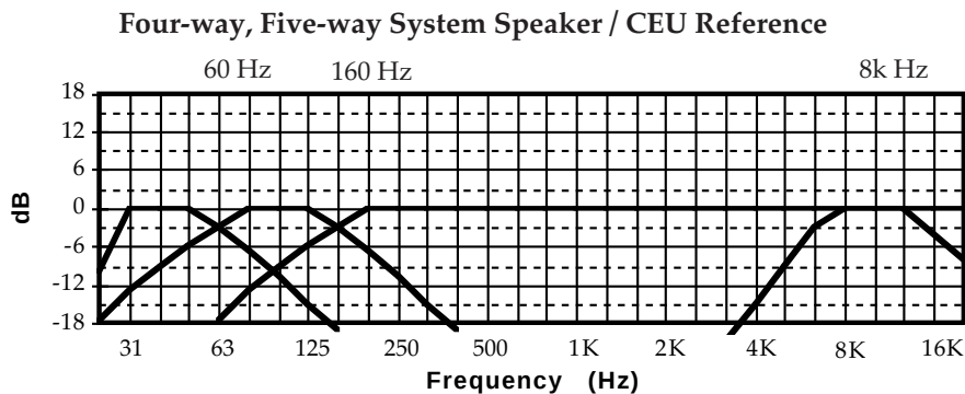
Five-way system frequency range chart.
