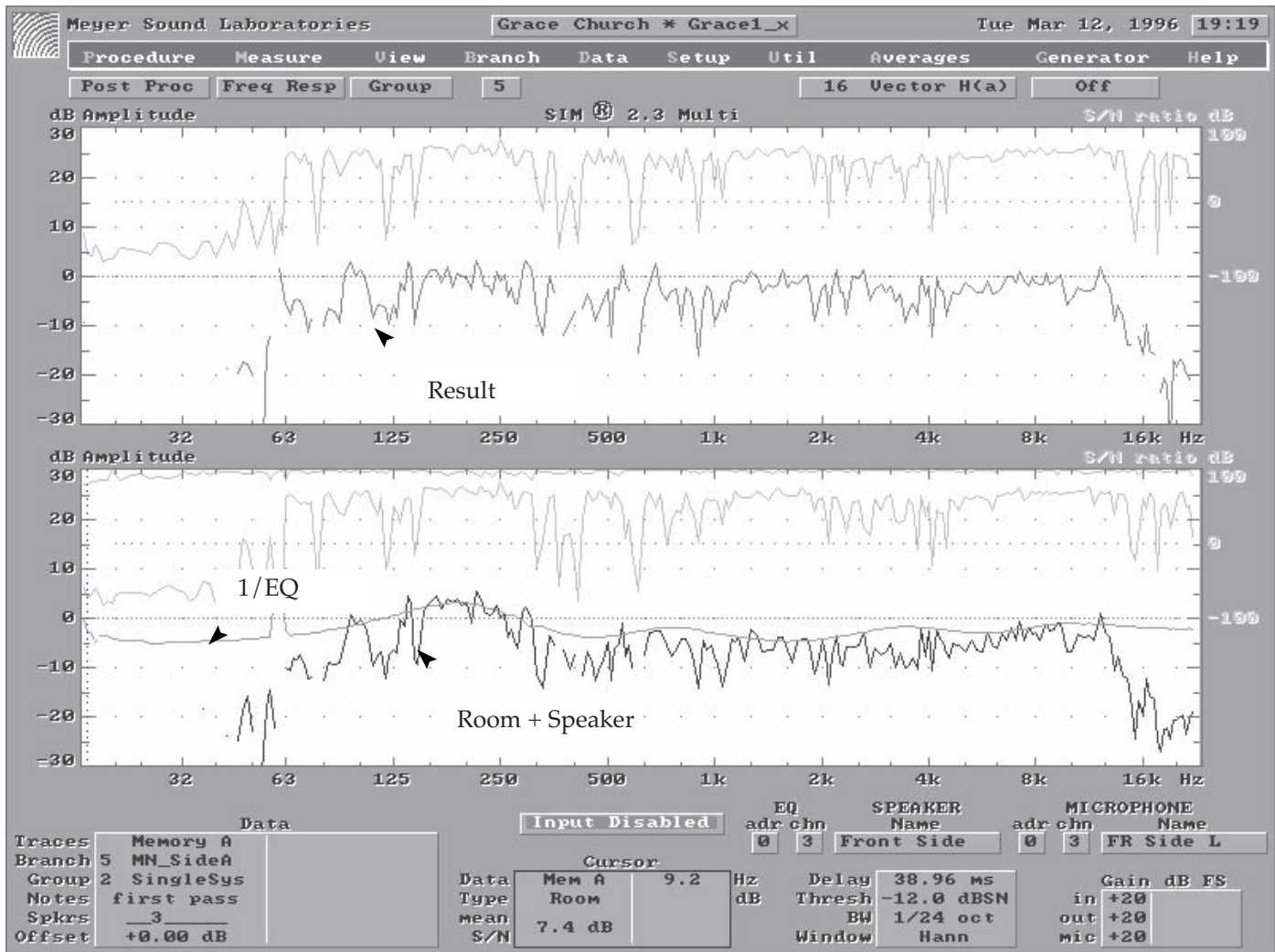
Fig 5.10h Equalizing the main side system.
