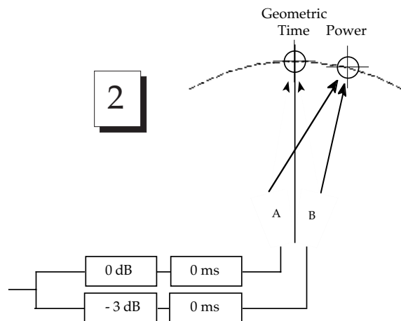
Fig 5.7h Delay tapering—Power center has moved.
