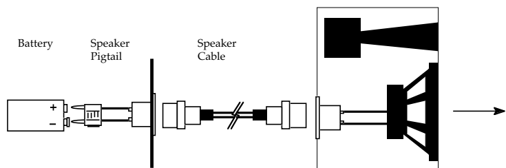
Fig 4.9a Battery polarity check.
