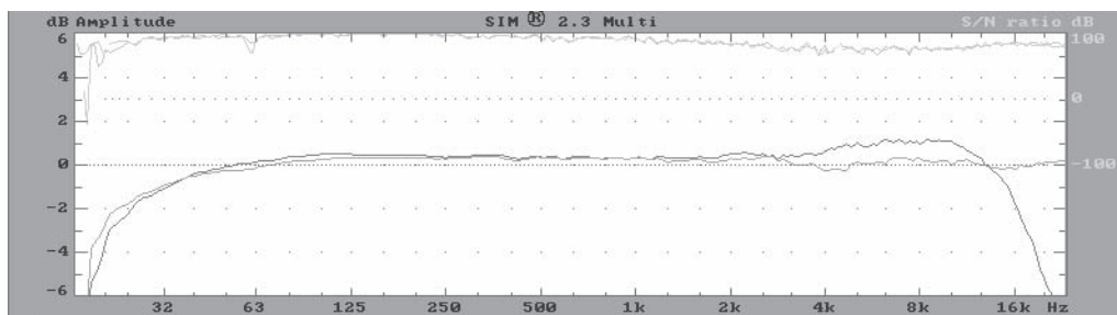
Fig 4.3b Comparison of two high-quality omnidirectional condenser mics. One of them costs three times as much as the other—Can you guess which one?
