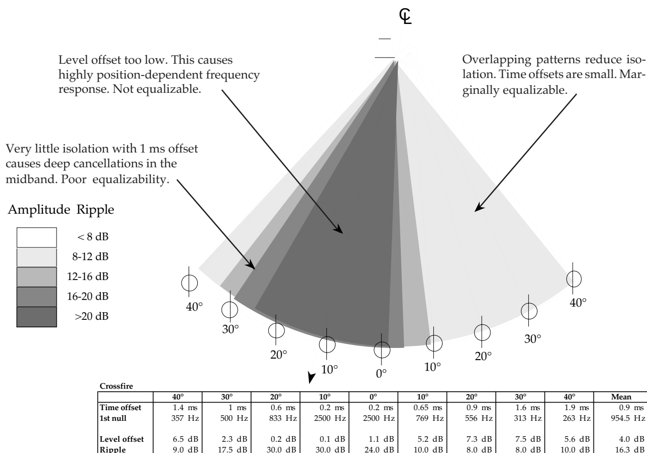
Fig 2.2u Crossfire array interaction.
