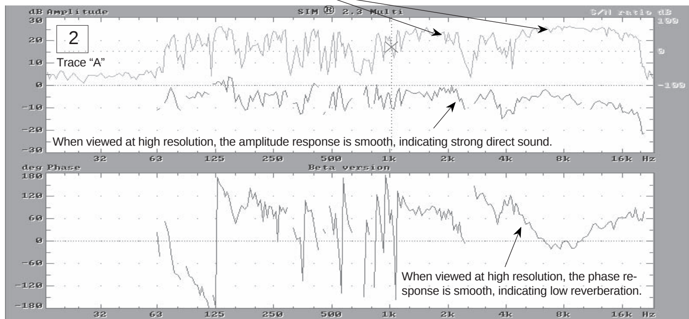
Fig 1.9k (2) High resolution view of amplitude, phase and S/N ratio of speaker "A" alone.
