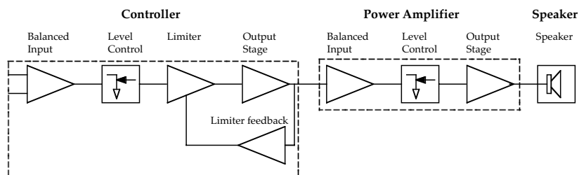
Fig 1.3f Predictive Limit signal flow block.
