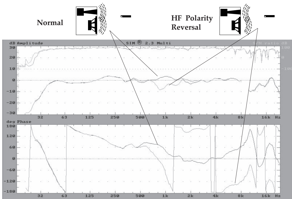
Fig 4.9f Polarity reversal of HF driver compared to a normal system.
