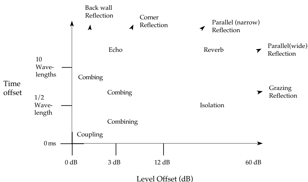
Fig 2.3a Tendencies for reflections to couple, combine and comb.
