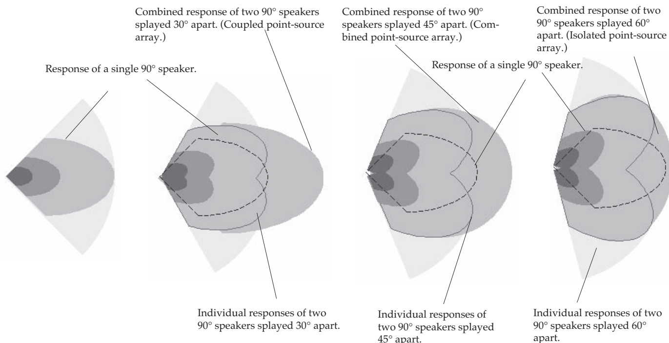
Fig 3.6h Coupled, combined and isolated point-source arrays.
