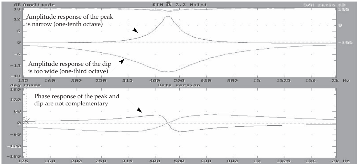
Fig 1.6j Peak and dip do not have the same bandwidth.
