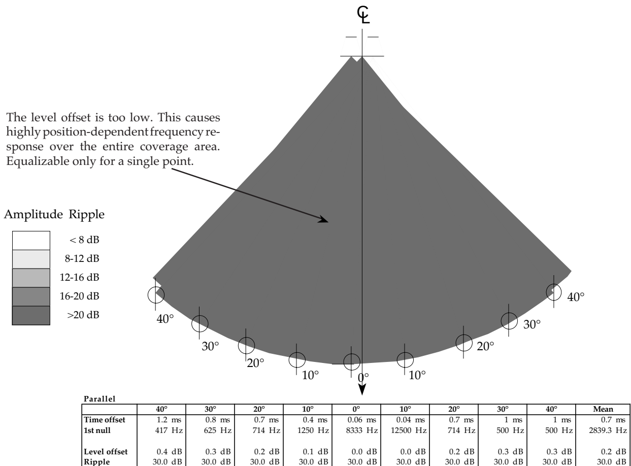
Fig 2.2s Parallel array equalizability.
