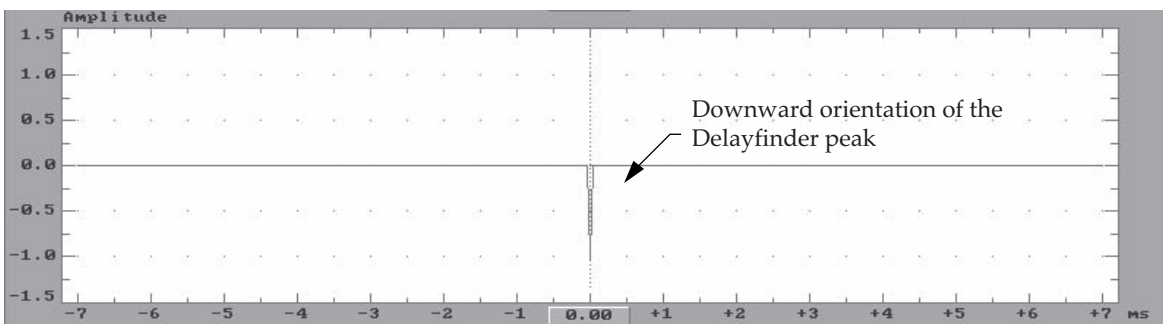
Fig 4.8d Polarity reversal of a balanced line. The peak of the delayfinder trace is pointing downward. This indicates that the system is "net inverting."
