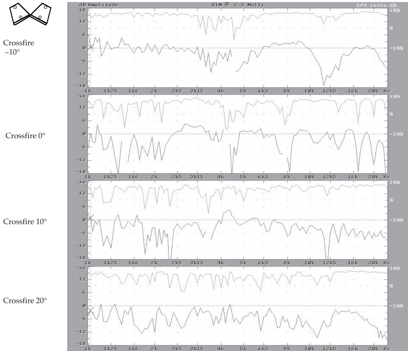
Fig 2.2v Crossfire array HF frequency response.
