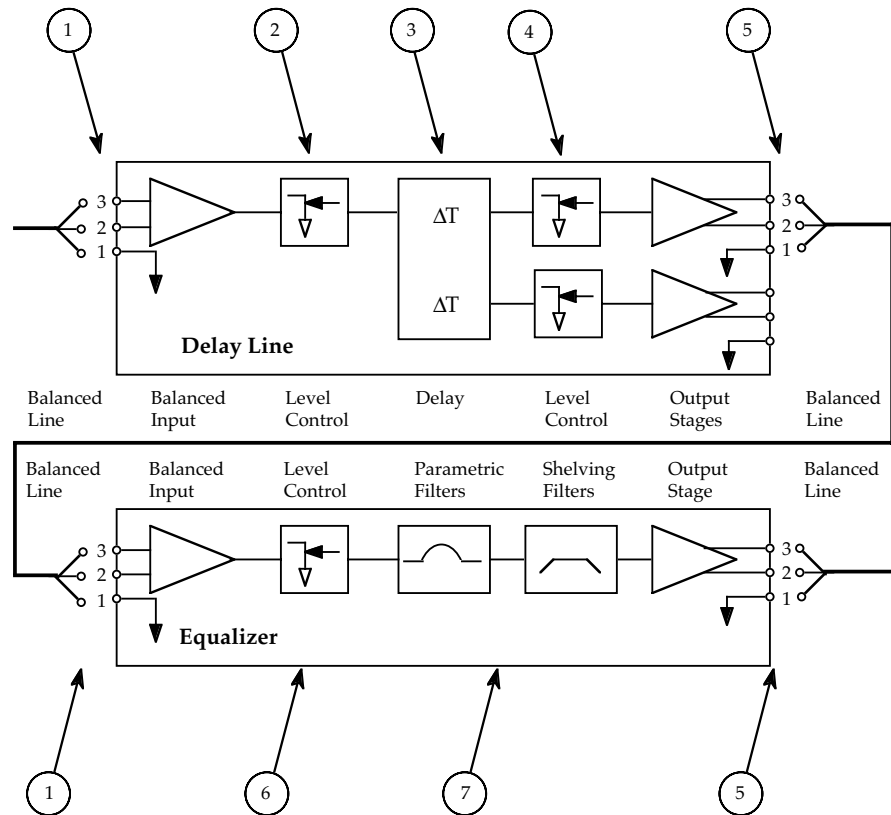
Fig 4.5a FOH rack verification.
