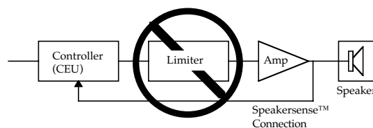
Fig 1.3a Additional limiters are not required for system protection and may actually compromise reliability as well as dynamic range.
