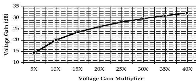
Fig. 1.4b Voltage gain multiplier versus dB gain.
