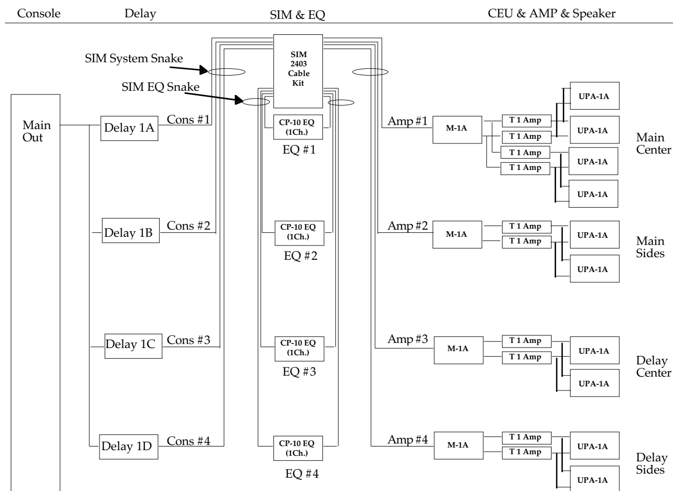
5.10c Flow block diagram of the system after SIM System II is patched in.
