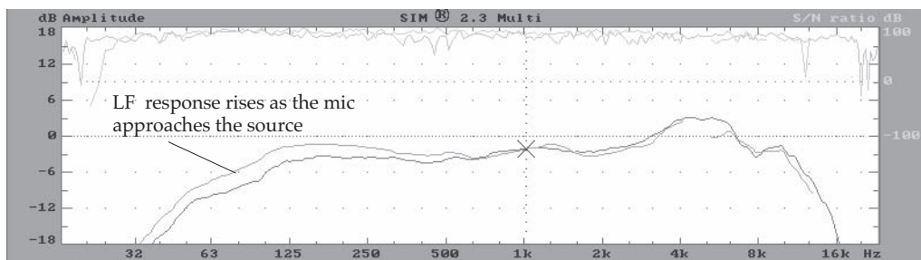
Fig 4.3c Cardioid mic exhibiting the "proximity effect" as it nears the source.
