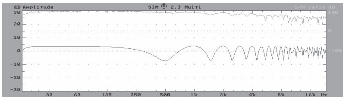
Fig 1.6d Linearly spaced comb filtering as created by the interaction of speakers with rooms and other speakers. See Section 2 for complete details. A parametric equalizer with adjustable center frequency, bandwidth and level is capable of creating a complement to this type of response.
