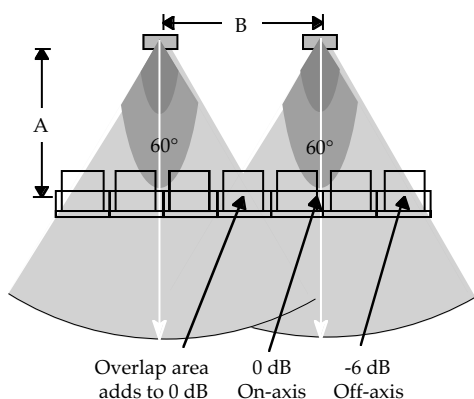
Fig 3.7g Speakers placed at proper relationship. For a 60° coverage angle A (the distance to the audience) will be equal to B (the enclosure spacing).
