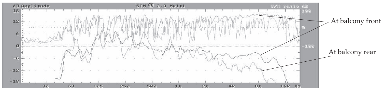
Fig 5.5d Speaker position example.
