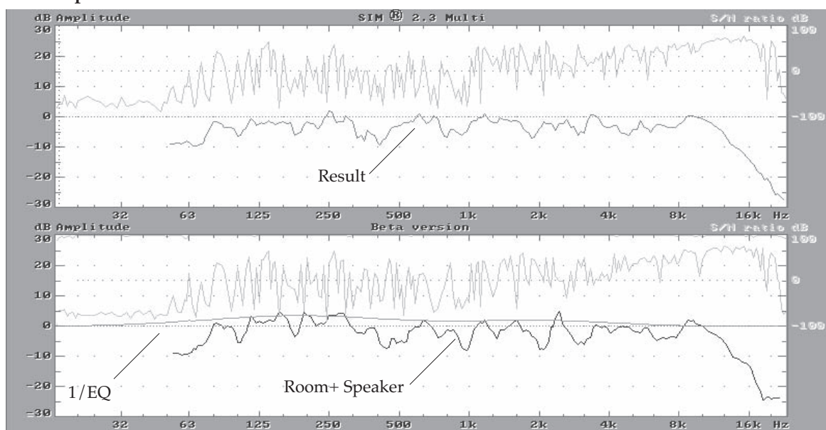
Fig 5.8e. This is the same system when equalized with SIM. The system response was greatly improved by equalizing the interaction of the speaker with the room and with each other, separate from the microphone.
