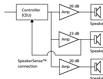
Fig 1.3j Sensing one of several amplifiers. Sense line connected to the correct amplifier.
