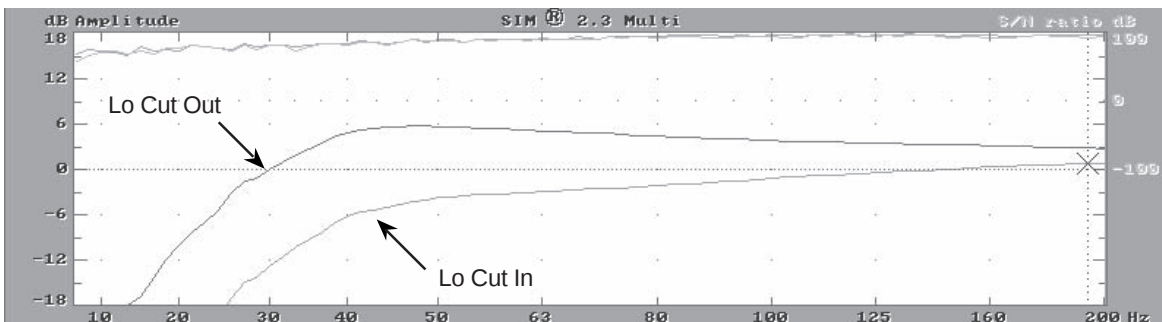
Fig 1.2m Lo Cut circuit response in the S-1 controller.
