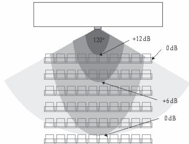
Fig 3.7f Point-source arrays or single wide coverage speakers are not recommended due to poor distribution level.
