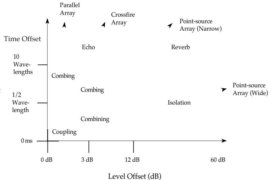
Fig 2.2f Tendencies of coupled arrays.
