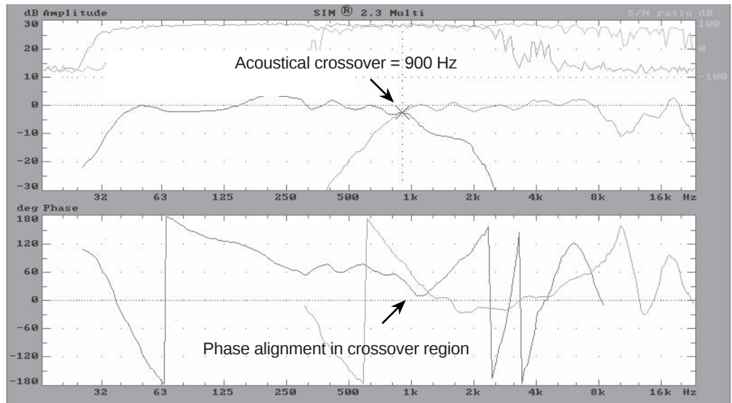
Fig 1.2b Acoustical response of the MSL-2A speaker system (with the S-1 CEU).
