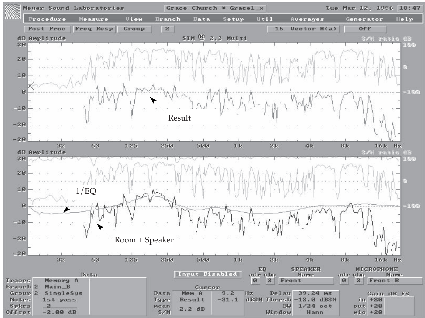
Fig 5.10f Equalization with SIM System II and the CP-10.
