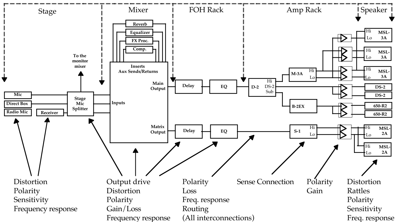
Fig 4.1a verification flow block.
