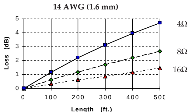
Fig. 1.7.i Cable loss over distance for 14 AWG (1.6 mm).
