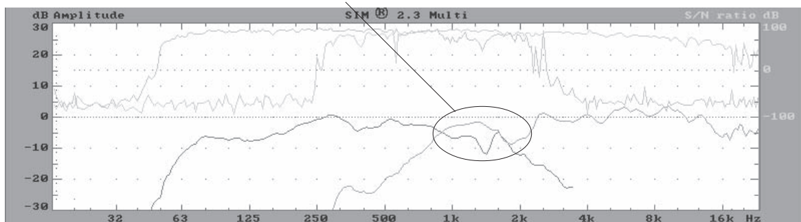
Fig 1.4i UPA-1C with unmatched voltage gains at crossover.
