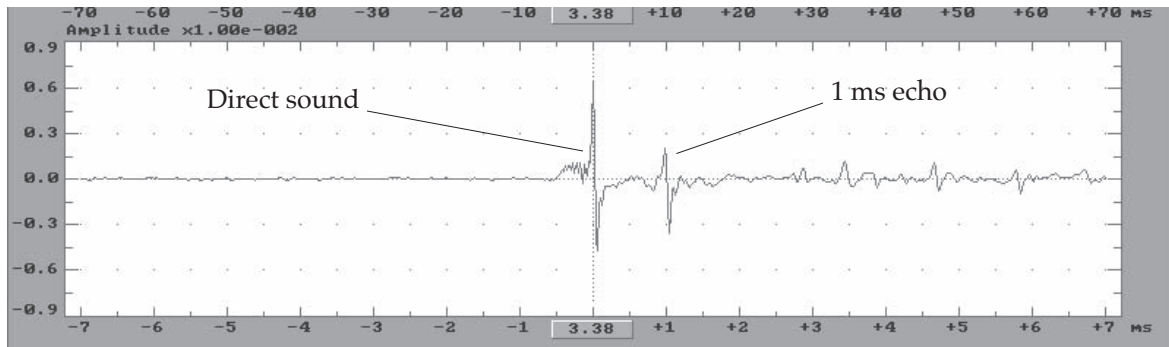
Fig 2.1l Identifying delay offset to find frequency response ripple.
