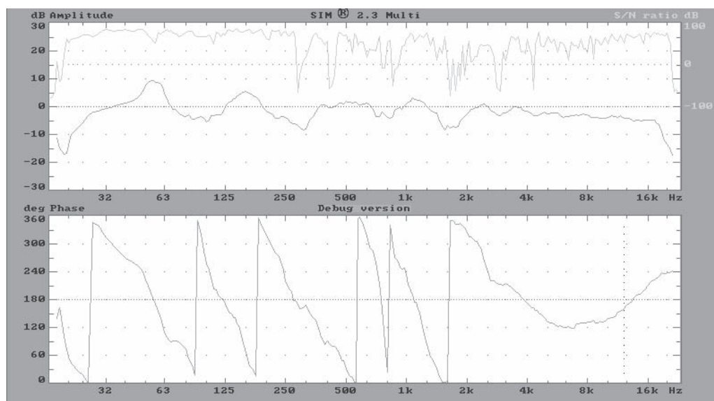
Fig 1.2g Competitor's system.
