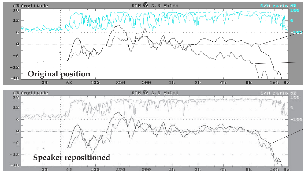
Fig 5.5b Speaker repositioning field example.
