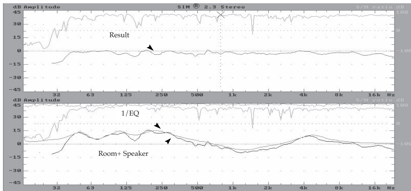
Fig 5.8c Group view of the three SIM transfer functions with the 1/EQ response. The process of creating a complementary response is aided by the visual inversion of the EQ trace. This allows you to simply match the equalizer response to the room+speaker response. This creates a flat response in the result.
