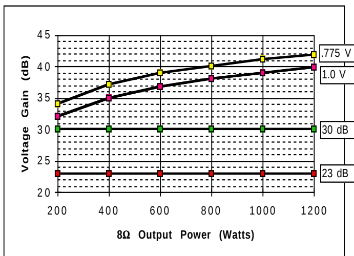
Fig. 1.4c Amplifier sensitivity versus dB gain.
