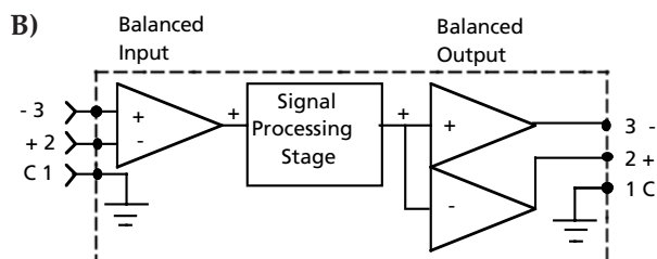
Fig. 1.7b Active balanced inputs and outputs.
