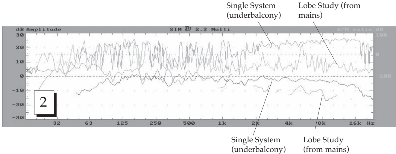
Fig 5.9b Lobe study analysis of the signal from the main system.
