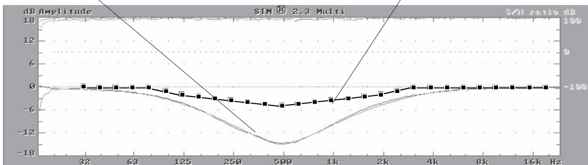
Fig 1.6e Contrasting a graphic equalizer and the CP-10 Parametric
