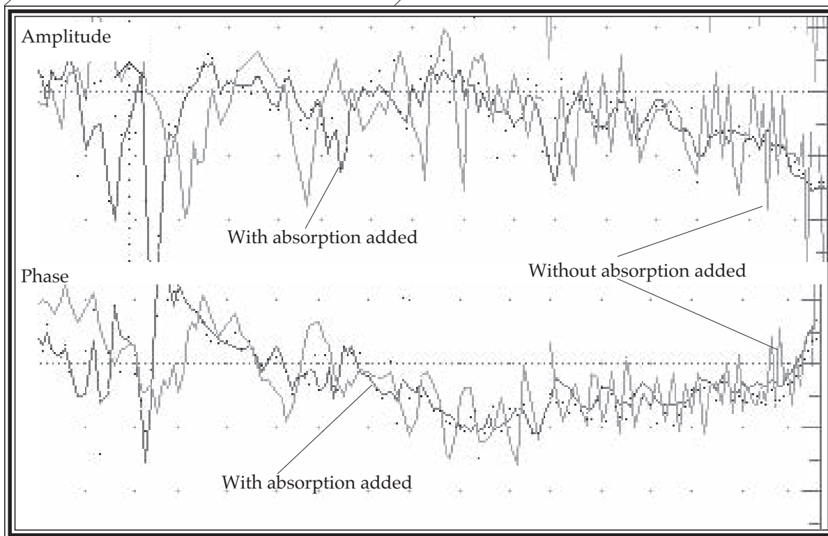
Fig 5.4b Effect of absorptive materials on frequency response.
