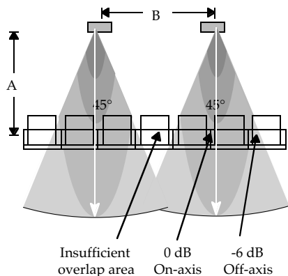
Fig 3.7i The speaker coverage angle is too narrow for the current spacing. There is a gap in coverage.
