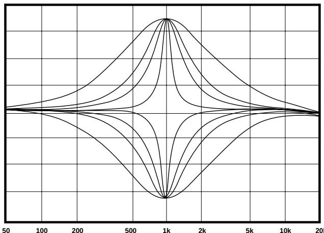
Fig 1.6a The CP-10 parametric equalizer section family of curves.
