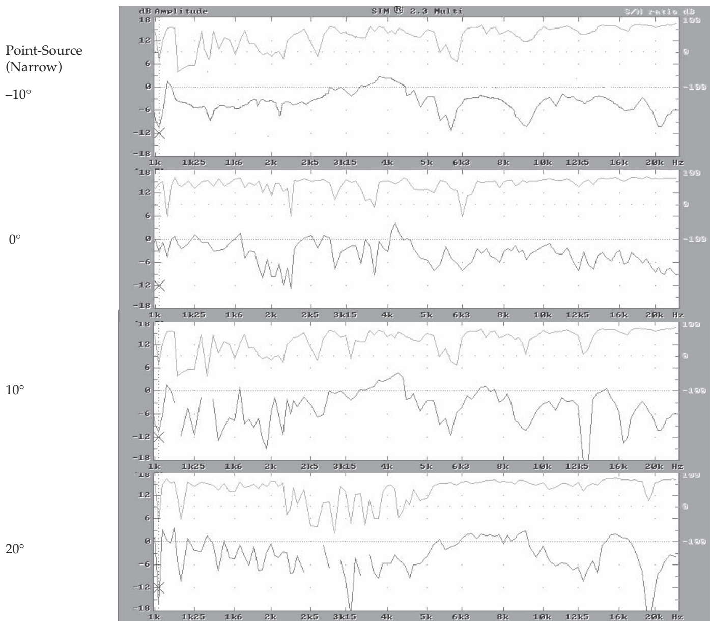
Fig 2.2k Narrow point-source array HF frequency response.
