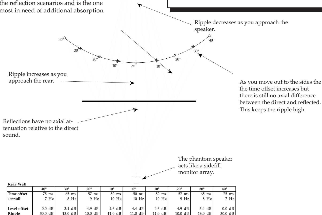
Fig 2.3d Rear wall reflection.
