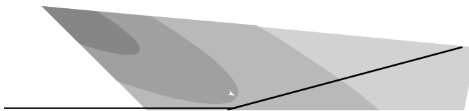
Fig 3.4j The speaker is aimed too low and will not achieve constant coverage. The level at the rear is 12 dB down from the main floor.
