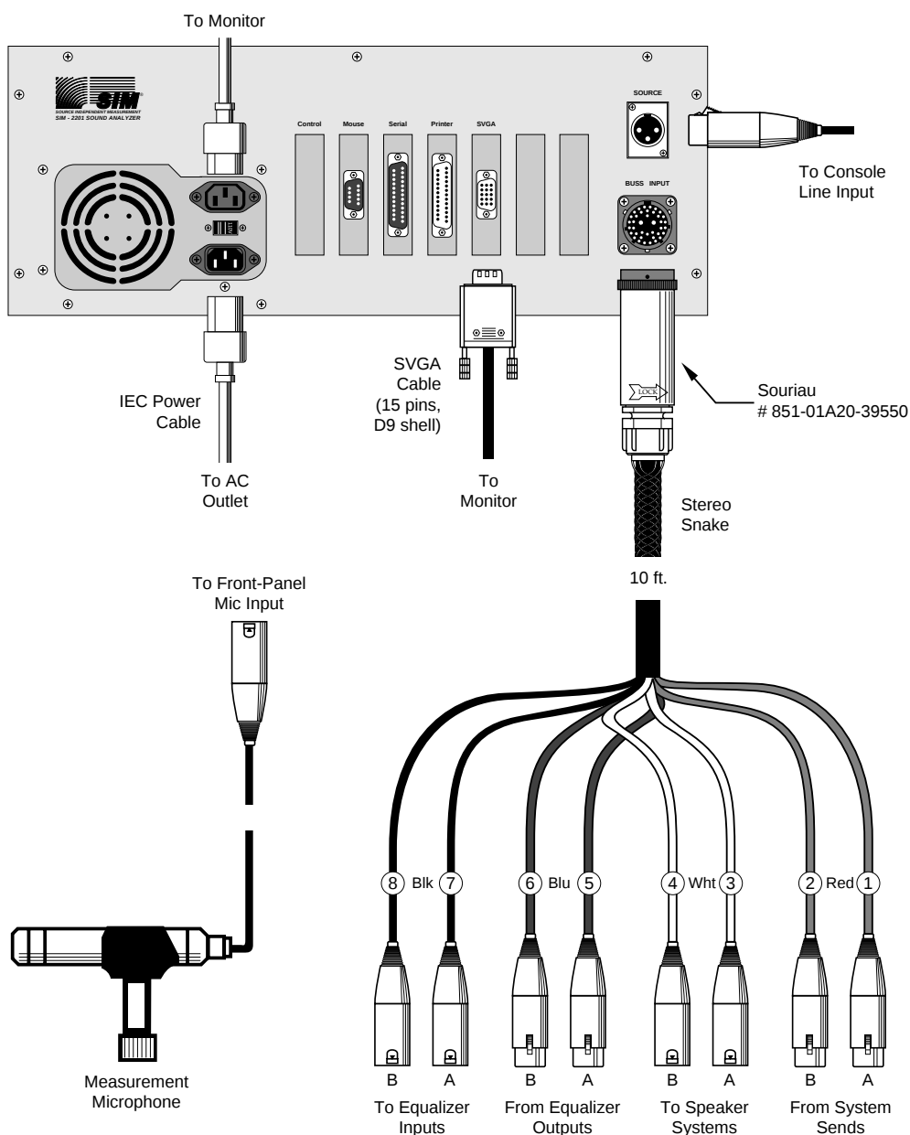
Fig 1.9q The v2.3 stereo hookup.
