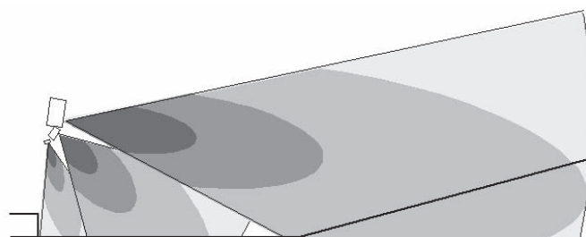
Fig 3.7c Traditional downfill.
