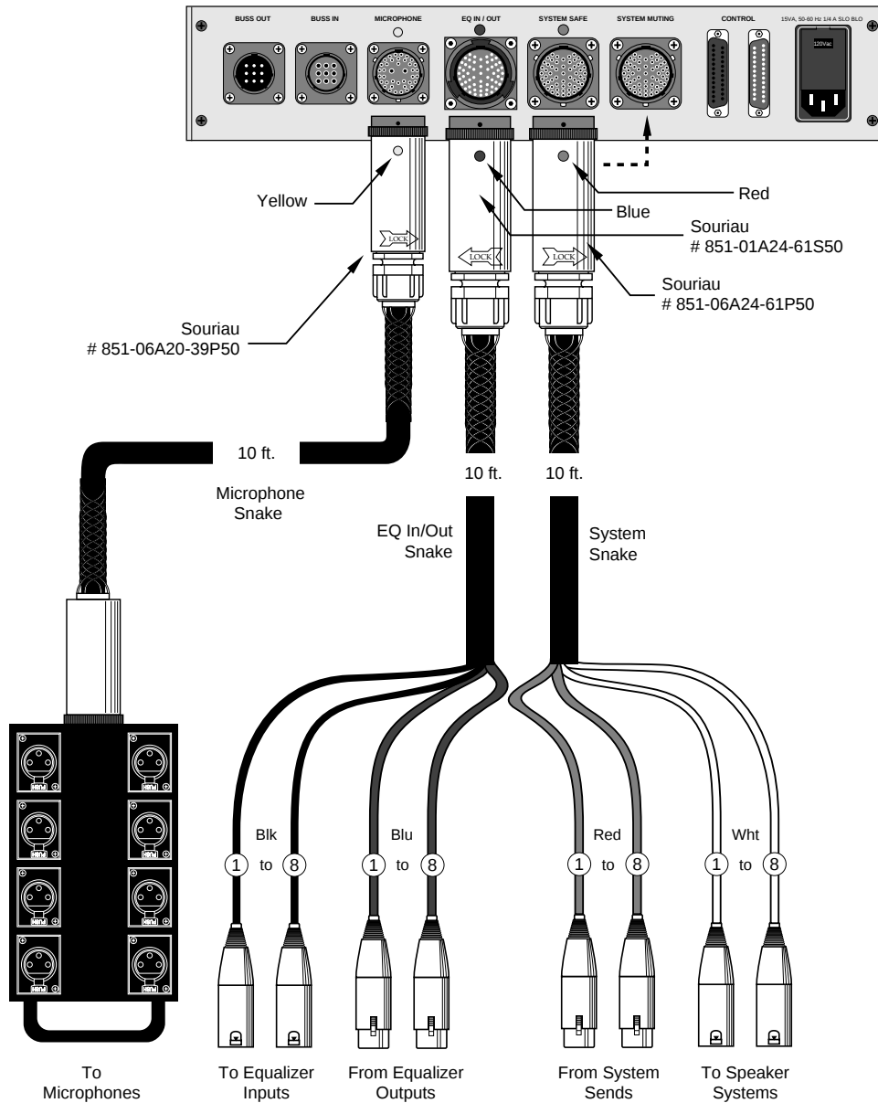
Fig 1.9r The v2.3m multichannel hookup.
