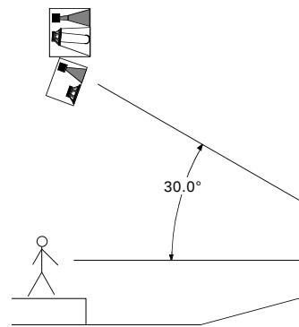
Fig 5.7a Vertical sonic image distortion.
