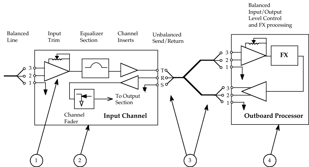
Fig 4.4a Input section verification.
