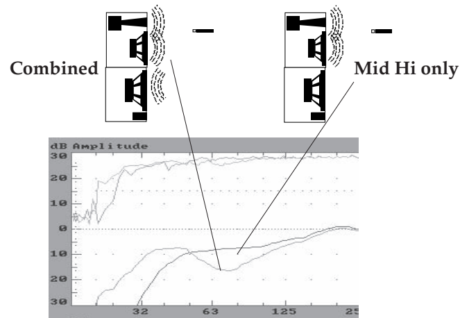
Fig 4.9k The combined response of the MSL-2A and MSW-2 subwoofer compared to the MSL-2A alone.
