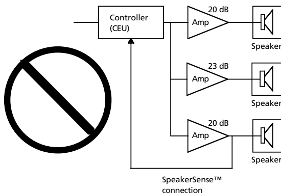
Fig. 1.3n Improper MultiSensing. Sense lines shorted together.
