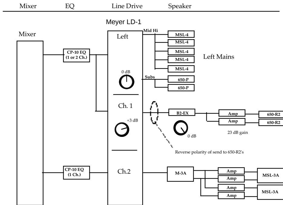
Fig 7.1a Combining externally-powered with self-powered speakers.
