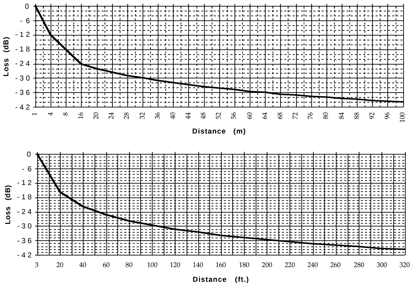
Fig 3.3b Propagation loss over distance (free-field) referenced to 1 meter SPL (in meters and feet).
