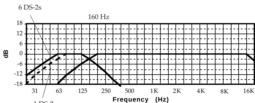
Three-way DS-2 system frequency range chart.
