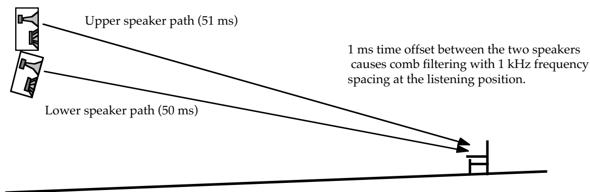
Fig 2.2a Elevation view of speaker interaction between an upper main and downfill system.
