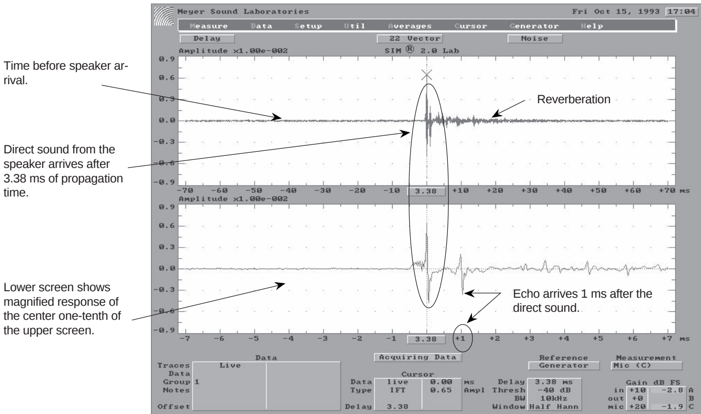
Fig 1.9h Reading the delayfinder screen.
