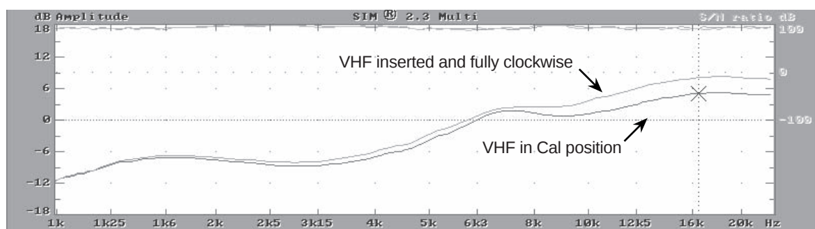
Fig 1.2n The VHF circuit response in the S-1 controller.
