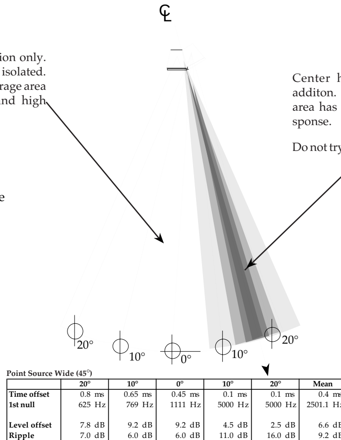
Fig 2.2p Wide point-source array interaction.
