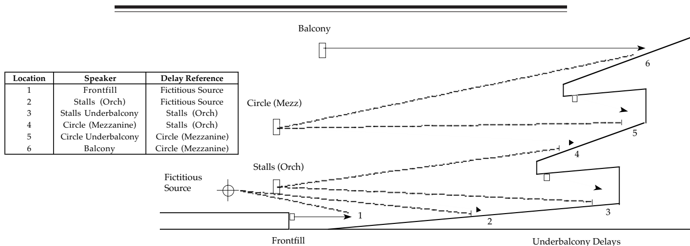
Fig 5.7d Musical theatre design example.
