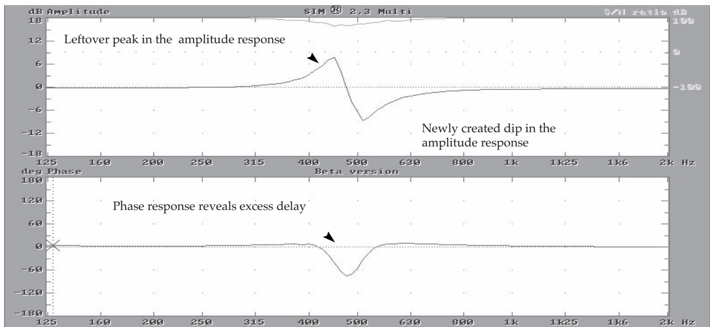
Fig 1.6i Result of error in center frequency.
