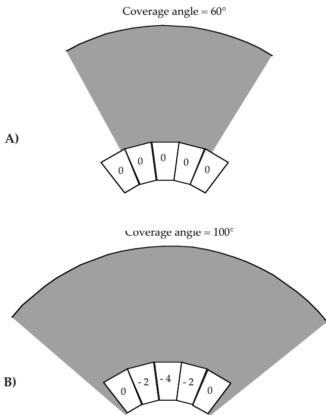
Fig 3.6i The effect of amplitude tapering on a tight-pack MSL-3A array.
