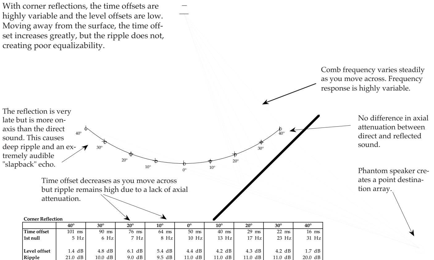
Fig 2.3e Corner reflection.
