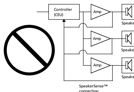
Fig 1.3k Sensing one of several amplifiers. Sense line connected to amplifier with lower gain.
