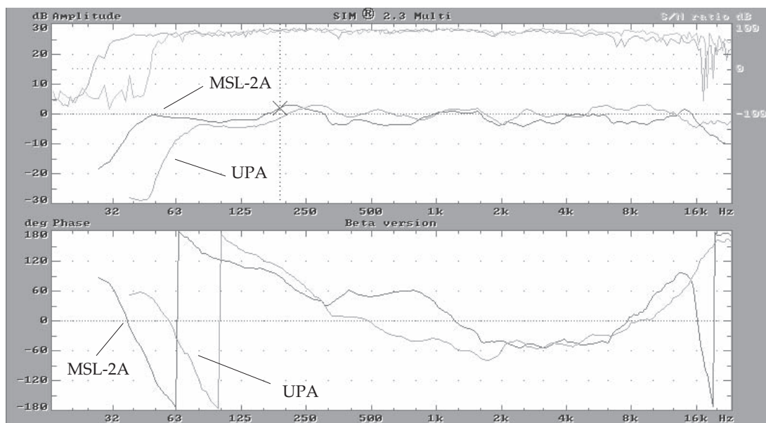
Fig 4.9h Comparison of the UPA and MSL-2A phase responses.
