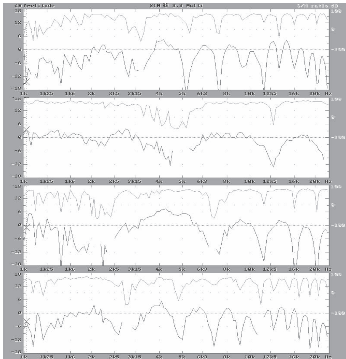
Fig 2.2t Parallel array HF frequency response.
