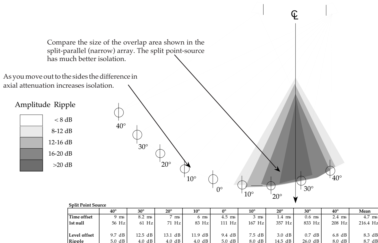
Fig 2.2y Split point-source array interaction.
