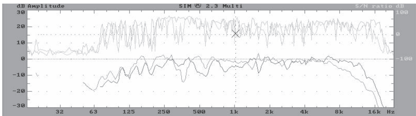
Fig 2.4c Air absorption causing HF loss over increased distance.
