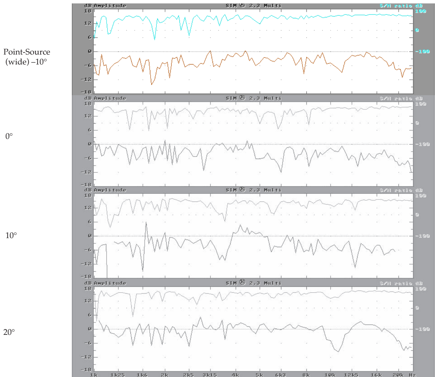
Fig. 2.2r Wide point-source array HF frequency response.
