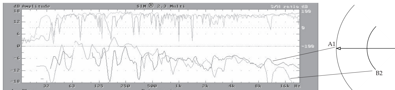
Fig 3.3e Comparison of on-axis far (A1) and off-axis near (B2).
