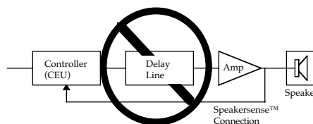
Fig 1.3b Delay lines should not be inserted here since it will disrupt the attack and release times of the limiters causing audible clipping and pumping.
