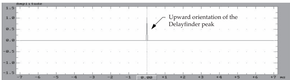
Fig 4.8b Normal balanced line. The peak of the delayfinder trace is pointing upward. This indicates a non-inverting line.
