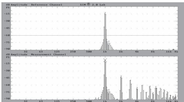
Fig 4.5b Distortion and maximum output testing with SIM.
