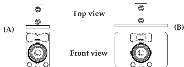
Fig 3.6e UPA-1C Enclosure design: (A) actual; (B) if the enclosure angle were equal to the coverage angle.
