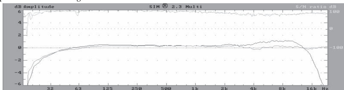
Fig 1.9a Frequency response of a typical Bruel & Kjaer Model 4007 microphone, compared to that of an alternative omnidirectional measurement mic suitable for multichannel sound reinforcement analysis.
