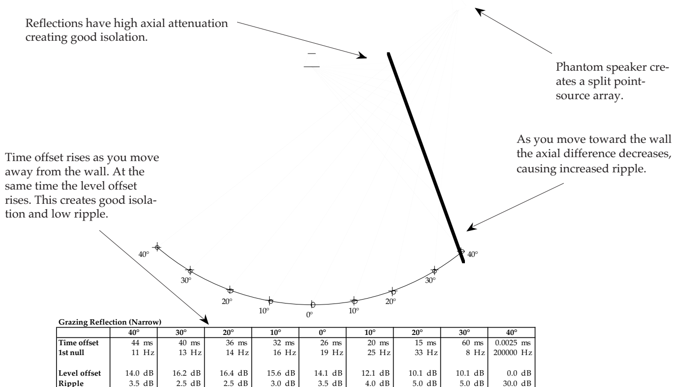
Fig 2.3b Grazing wall reflection.
