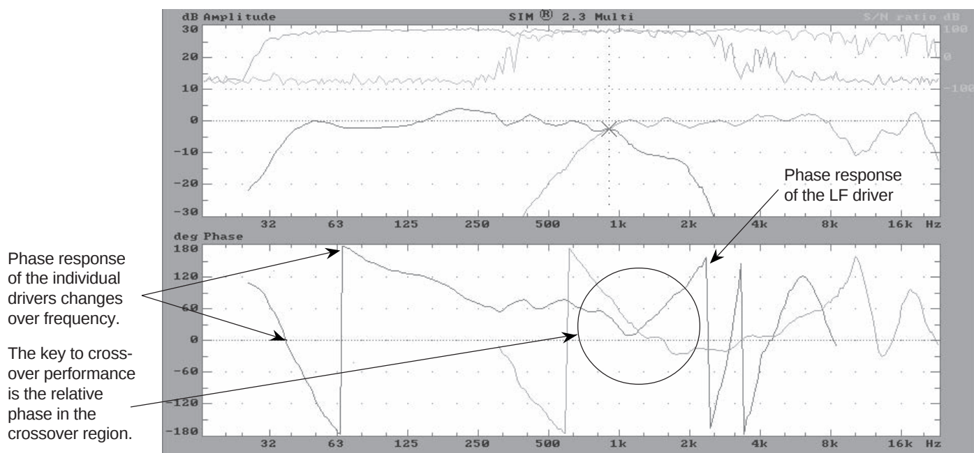
Fig 1.9e The phase response of the acoustical crossover of the MSL-2A loudspeaker. Notice the speakers are "in phase" through the crossover region, yet other regions are "out of phase." A simple "in phase" or "out of phase" reading is not valid for such a system.
