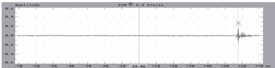
Fig 5.7e Delayfinder data indicates that 56 ms of delay must be added to this system. This is seen by the position of the impulse.
