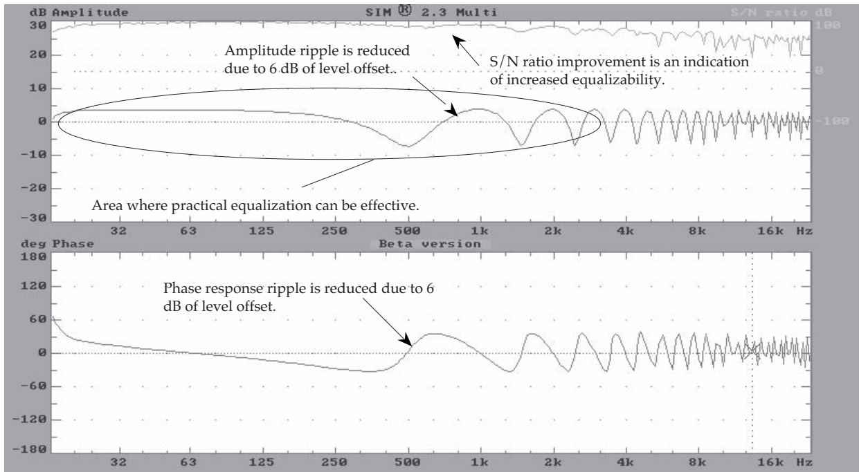
Fig 2.1i Comb filtering with 1 ms time offset between signals with 6 dB level offset.
