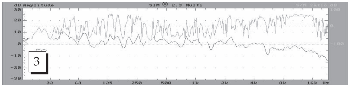
Fig 5.9c Combined system analysis of the main and delay systems.
