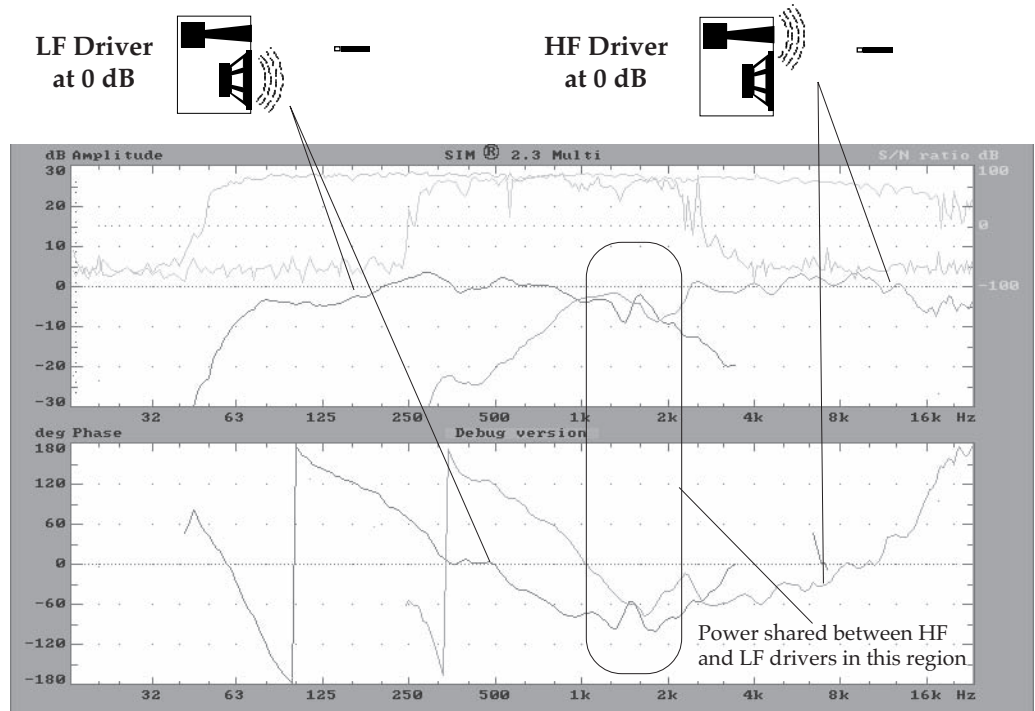
Fig 4.10a Normal crossover of the UPA-1C. Both amplifiers have the same gain.
