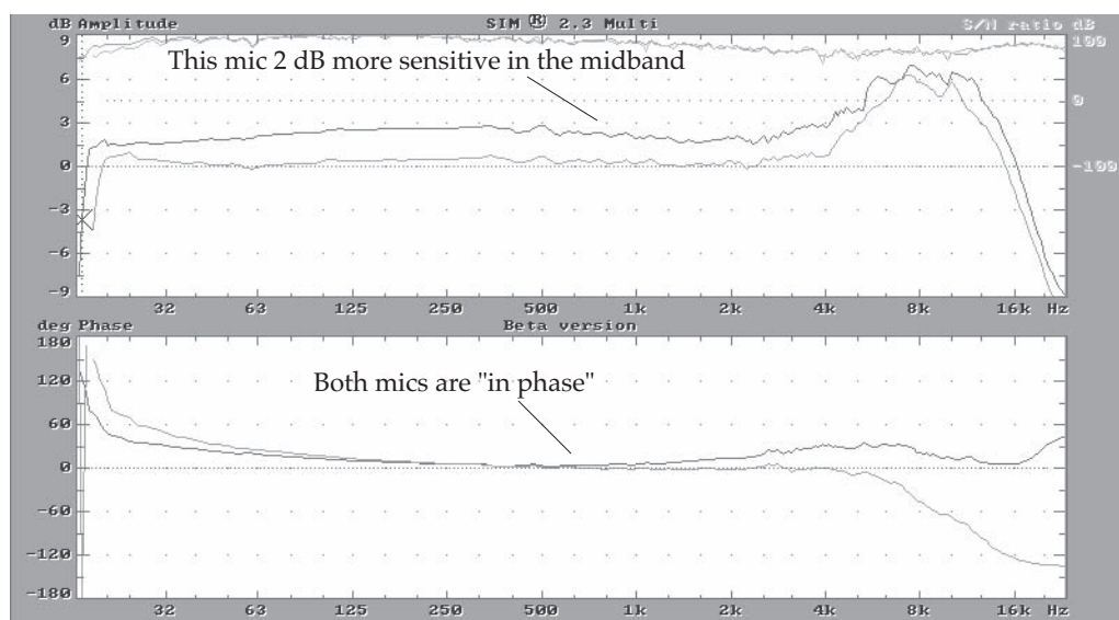
Fig 4.3d Microphone matching.
