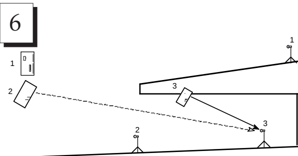
External delay alignment of the underbalcony.
