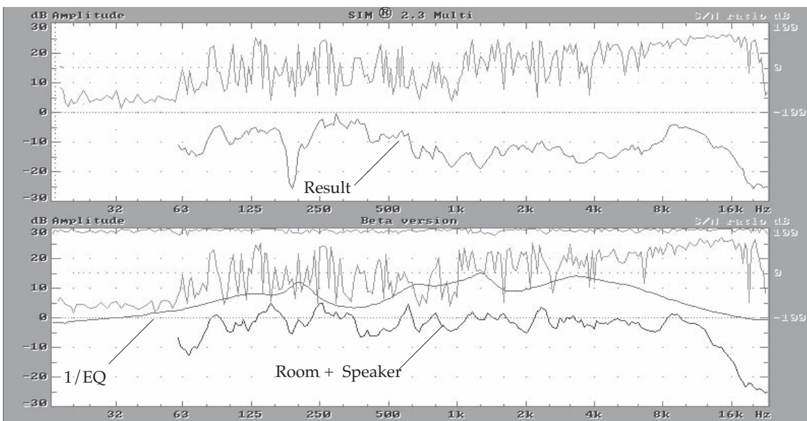
Fig 5.8d. The data here is of a poorly equalized sound system. The system was equalized primarily to suppress feedback of a podium mic. This was one of six subsystems, all of which had similarly set equalizers. The podium mic was not the only signal passing through this system. All other signals (such as the CD we listened to) sounded awful. The podium mic should have been equalized separately. When viewing the data notice that the inverse EQ does not at all correspond to the room+speaker response. The result response was worse than the original room+speaker response.
