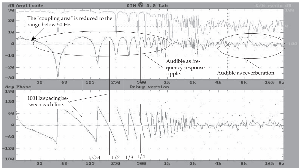
Fig 2.1g Comb filtering with 10 ms time offset between signals with 0 dB level offset.
