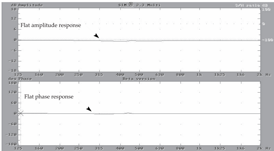
Fig 1.6g The result of complementary phase equalization. Amplitude and phase responses are flat.
