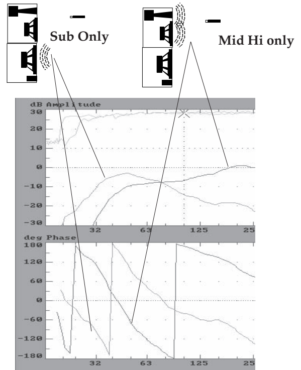
Fig 4.9j Subwoofers and mid-ranges with divergent phase responses.
