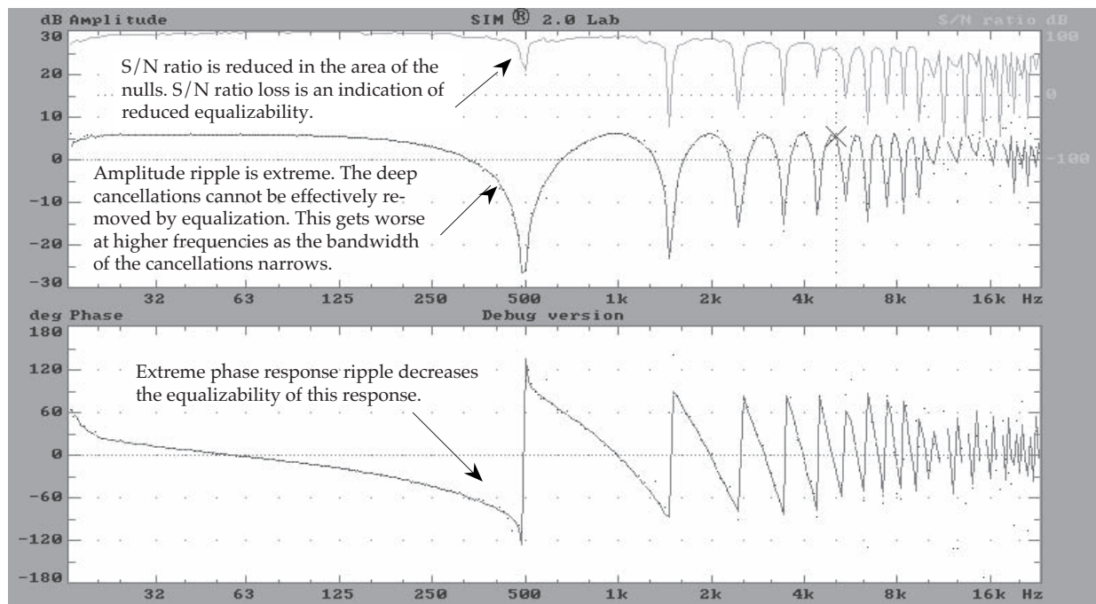
Fig 2.1h Comb filtering with 1 ms time offset between signals with 0 dB level offset.
