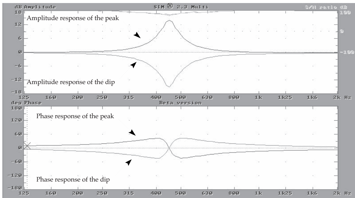
Fig 1.6f Peak and dip are complementary in amplitude and phase. The center frequency, bandwidth and level of the peak and dip are matched.
