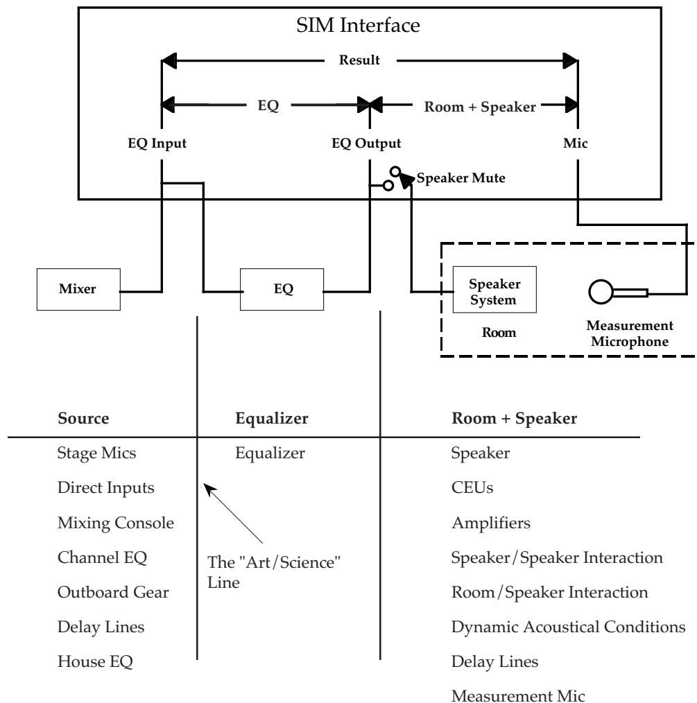
Fig 5.2a SIM interface patched into a sound system.
