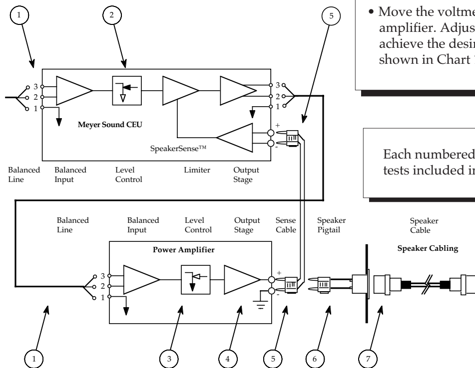
Fig 4.6a Amplifier rack verification.
