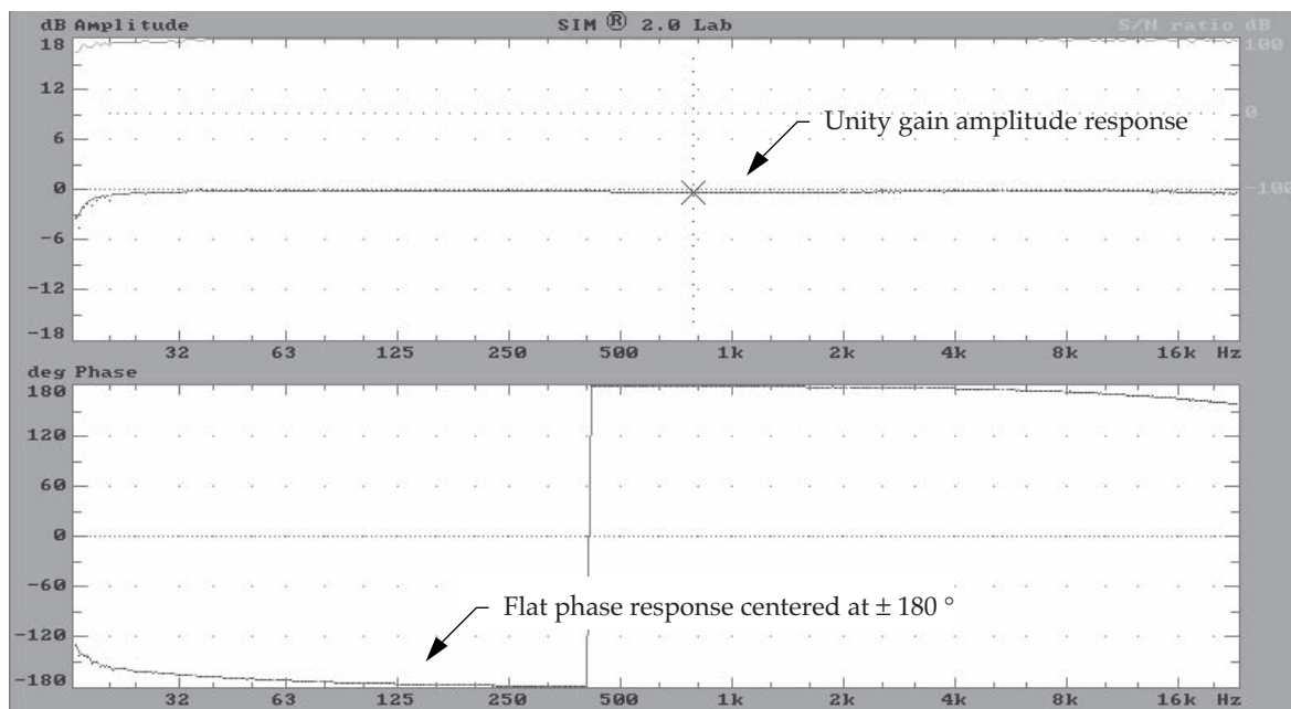
Fig 4.8c Polarity reversal of a balanced line. The amplitude trace is unaffected, however, the phase trace is centered at 180^\circ . This indicates a polarity inversion.
