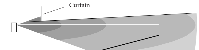
Fig 3.4l An eyebrow curtain prevents HF leakage onto the roof, while maintaining an optimal angle.
