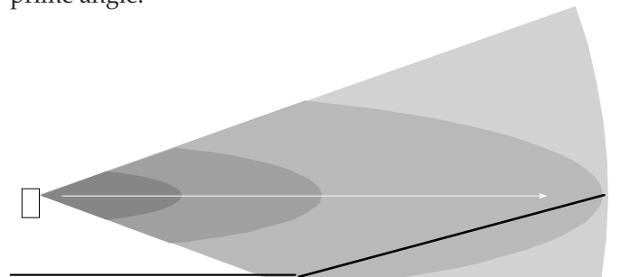
Fig 3.4k An elevation view of a speaker aimed for constant coverage. All the seats in the coverage area are near the 0 dB contour.
