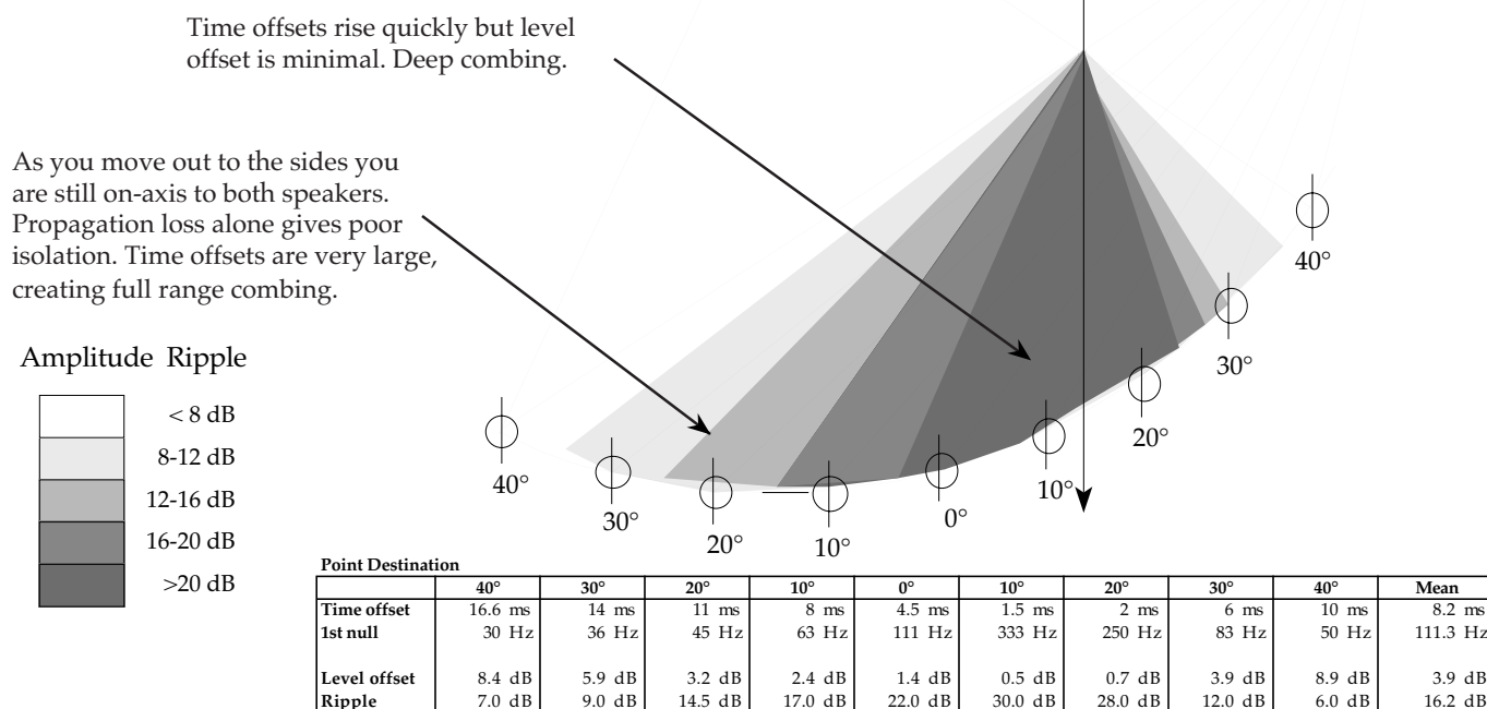
Fig 2.2z Point-destination array interaction.
