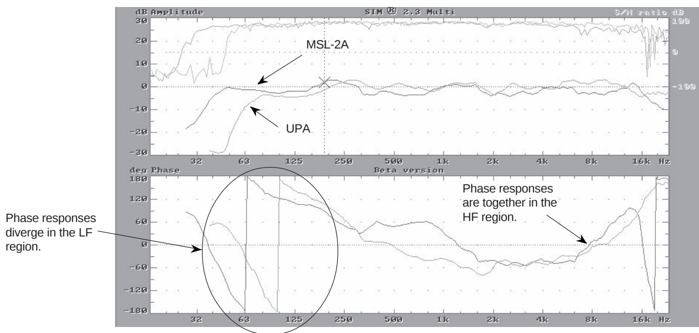
Fig 1.9f The phase responses of the UPA-1C and MSL-2A. The speakers are matched in phase throughout the HF range. However, as the LF cutoff is approached the phase responses diverge. Which of these is "in phase" and which is "out?" A phase popper could give conflicting results depending on which frequency range it reads. This difference in phase response becomes critical when subwoofers are added to these systems.
