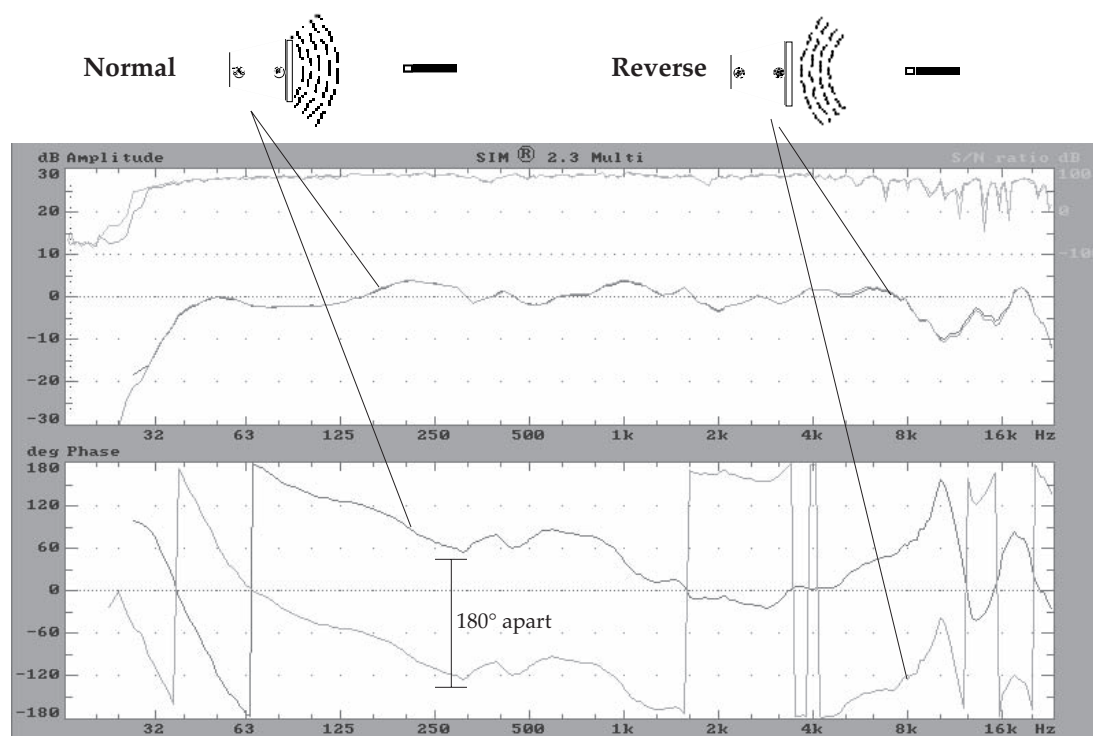
Fig 4.9c Polarity reversal of both the HF and LF drivers compared to that of a normal system. The amplitude response is identical. The phase response shows a difference of 180^\circ at all frequencies. The sound of these two speakers will be the same. The only difference is how they combine with other speaker systems.
