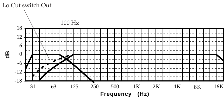
Three-way system frequency range chart.
