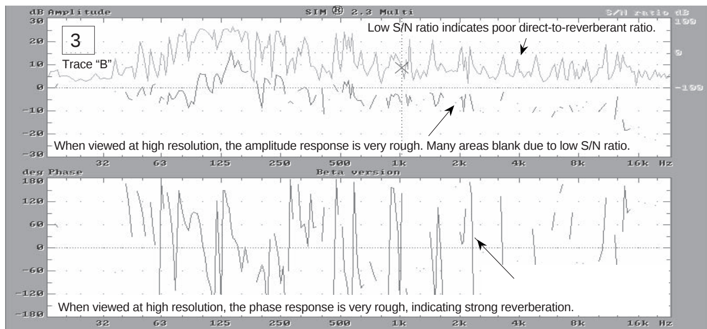
Fig 1.9l (3) High-resolution view of amplitude, phase and S/N ratio of speaker "B" alone.
