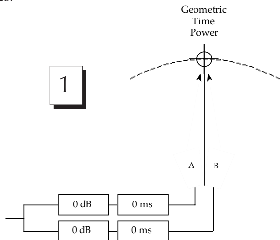
Fig 5.7g Delay tapering—All centers are together.
