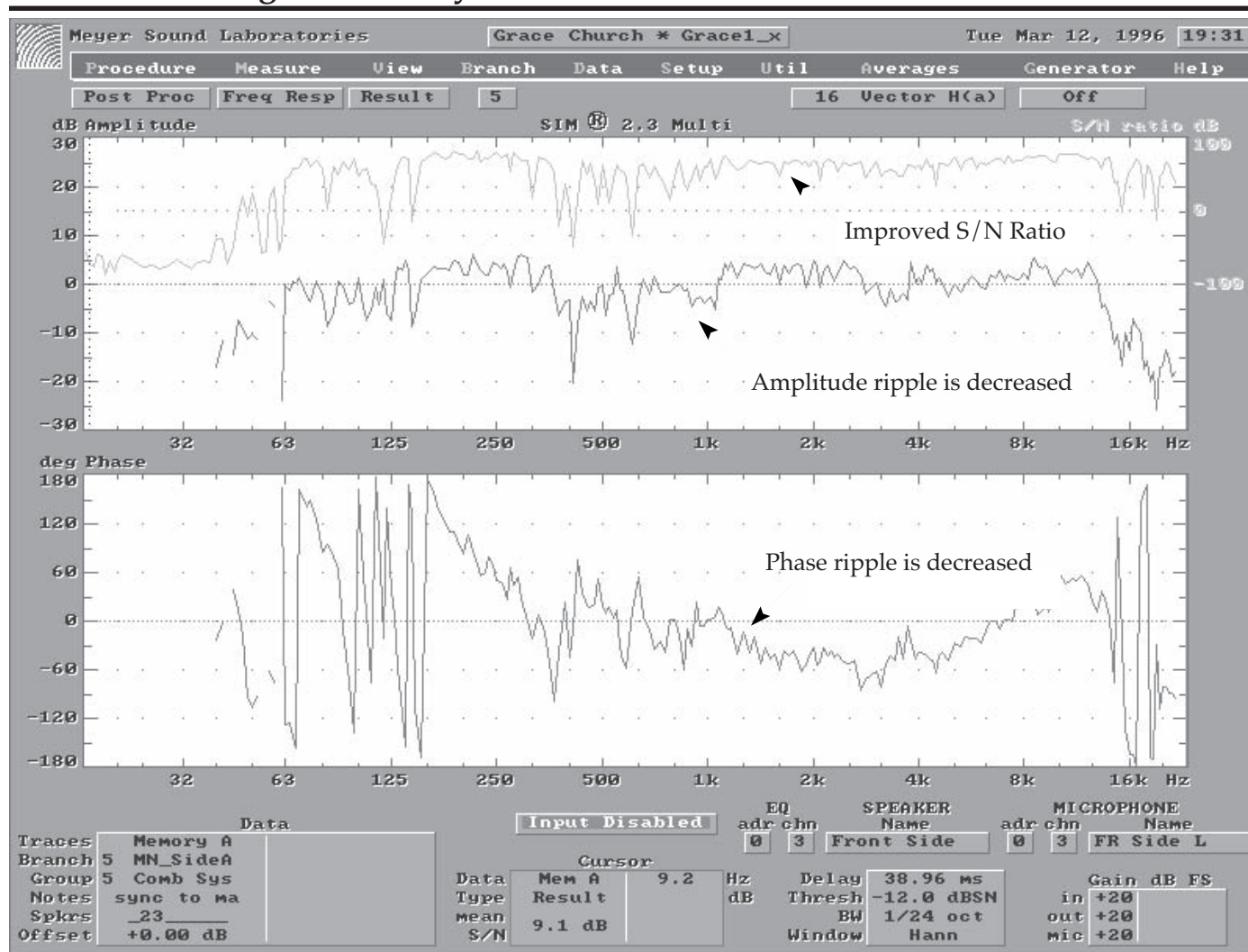
Fig 5.10k Delay tapering of the side system.
