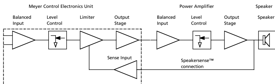
Fig 1.3c SpeakerSense signal flow block.
