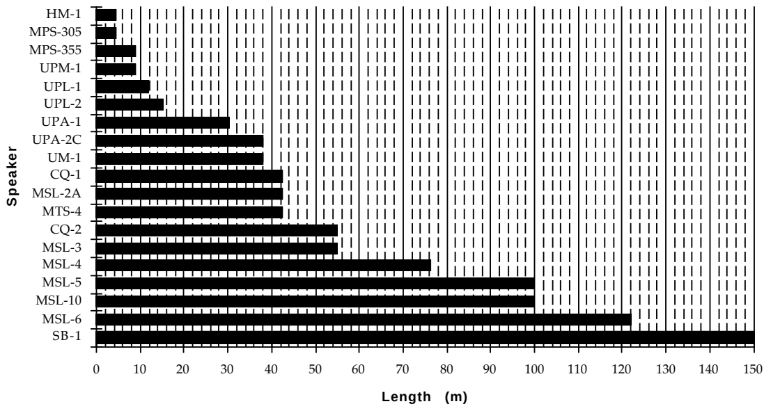
Fig 3.7k Delay speaker reference (meters).
