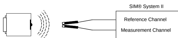
Fig 4.3a Mic comparison measurements using SIM System II.
