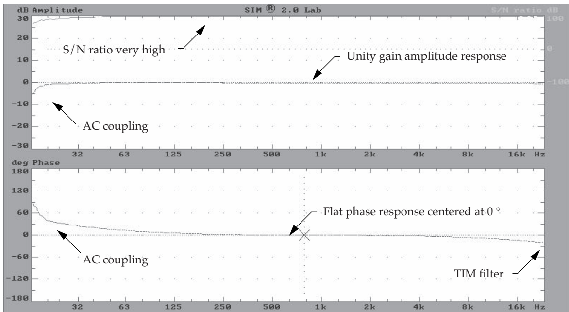
Fig 4.8a Normal balanced line. The amplitude trace shows unity gain. The phase trace is centered at 0°. This indicates a non-inverting polarity. The AC coupling and transient inter-modulation (TIM) filters will only be found on active devices and transformers (not cables).
