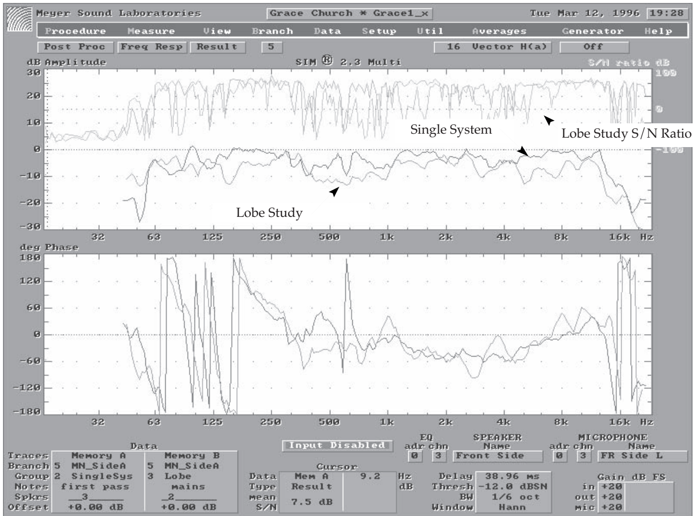
Fig 5.10i Checking for isolation between the main and side systems.
