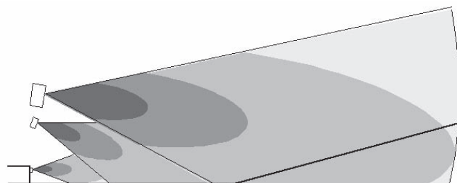
Fig 3.7d Downfill combined with frontfill.
