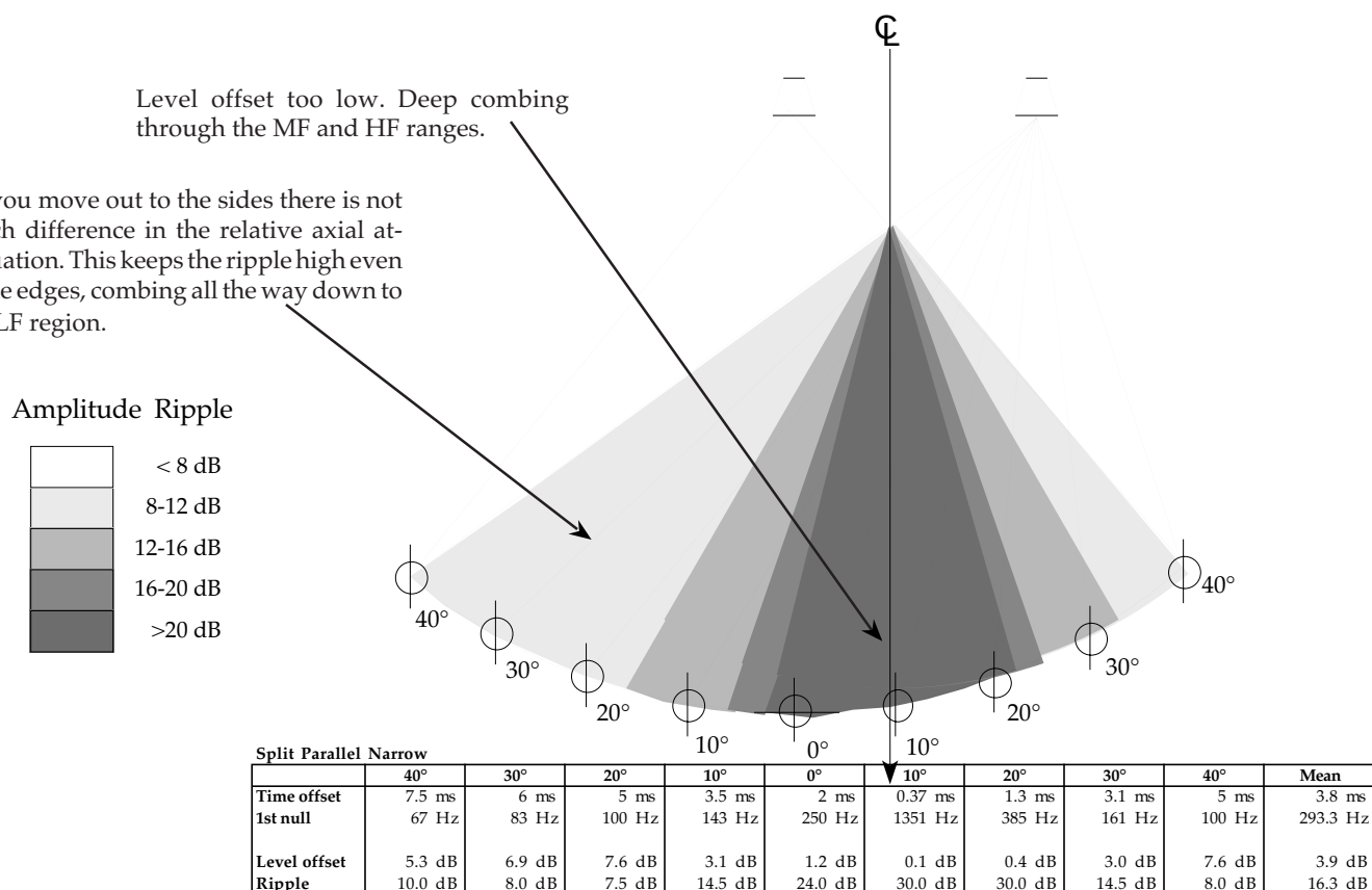
Fig 2.2w Split-parallel (narrow) array interaction.
