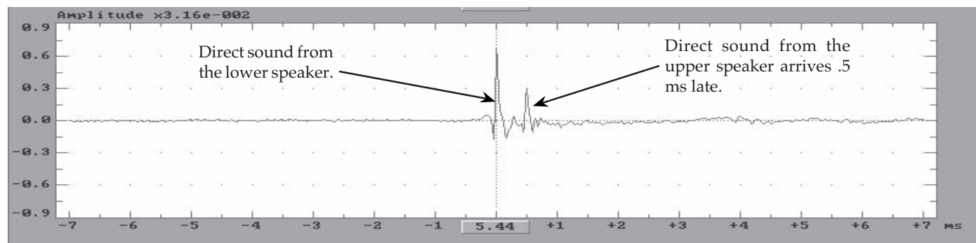
Fig 2.2c Delayfinder display of the arrivals of the two speakers.
