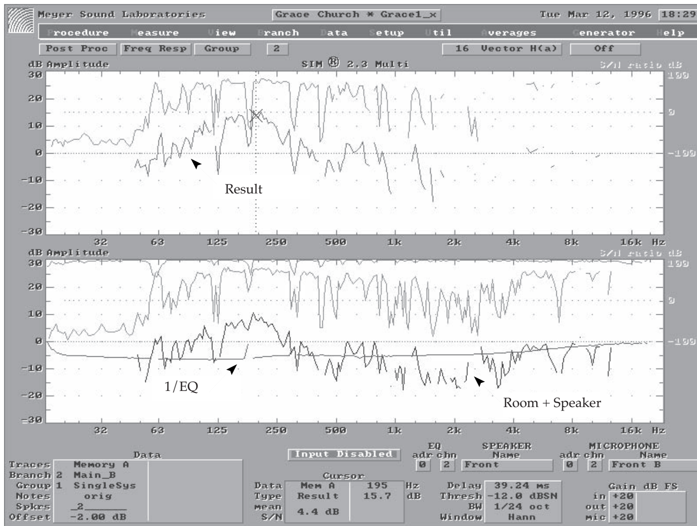
Fig 5.10e Original equalization of the main cluster.
