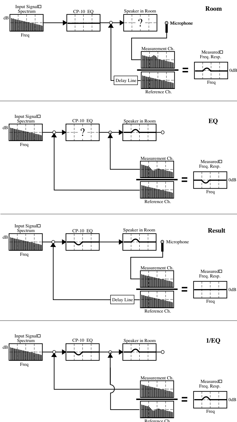
Fig 5.8a Room/EQ/Result Flow Block.
