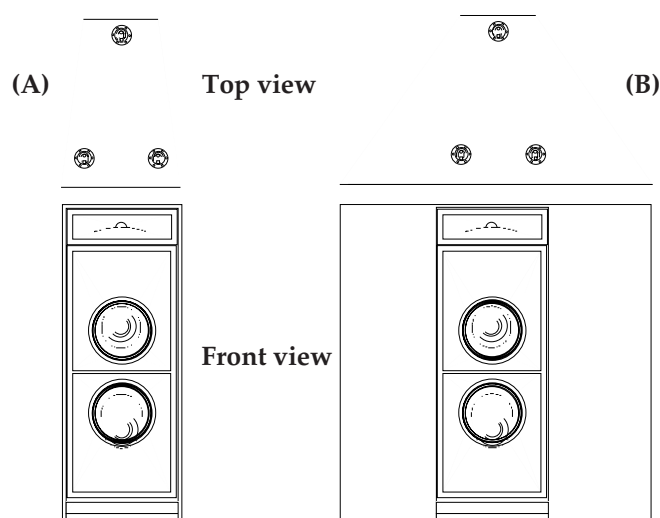
Fig 3.6f MSL-3A Enclosure design: (A) actual; (B) if the enclosure angle were equal to the coverage angle.
