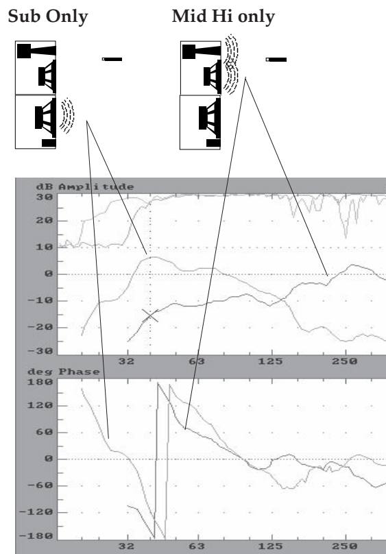
Fig 4.9i Subwoofer and mid-ranges with matched phase responses.
