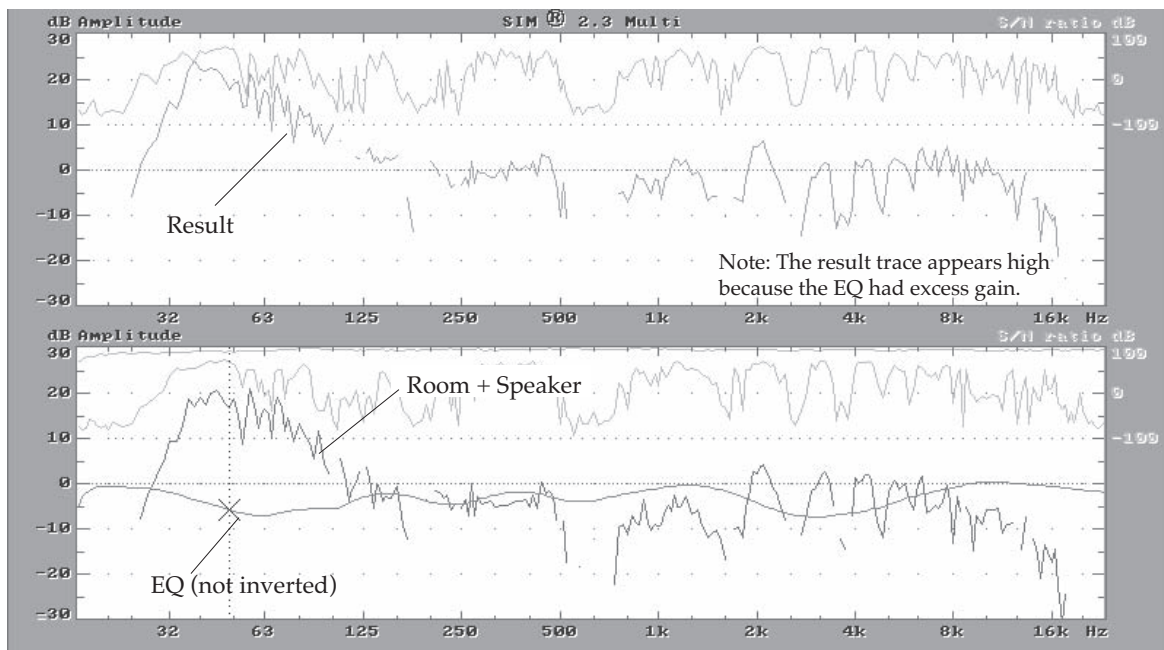
Fig 5.8g Is this system flat?
