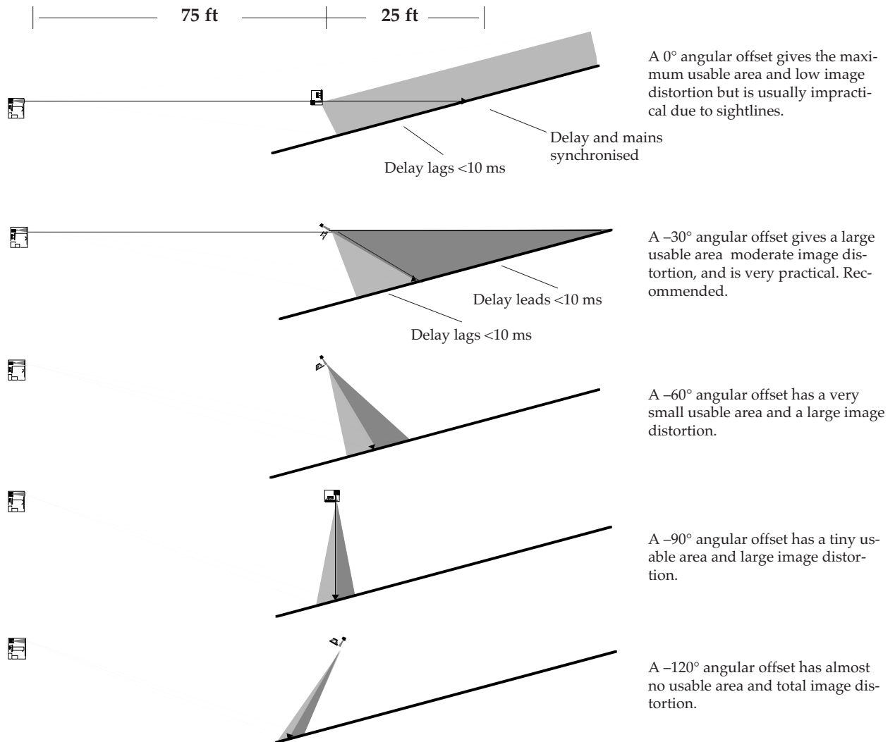
Fig 3.7m Usable vertical angle for distributed delays.
