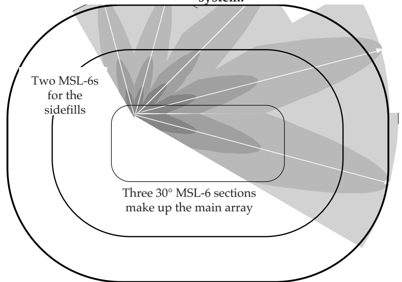
Fig 3.4q Plan view of an example of an arena concert system.
