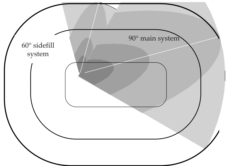
Fig 3.4p Plan view of an example of an arena concert system.
