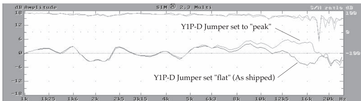
Fig 1.8h UPA-1C response with Y1P-D network.
