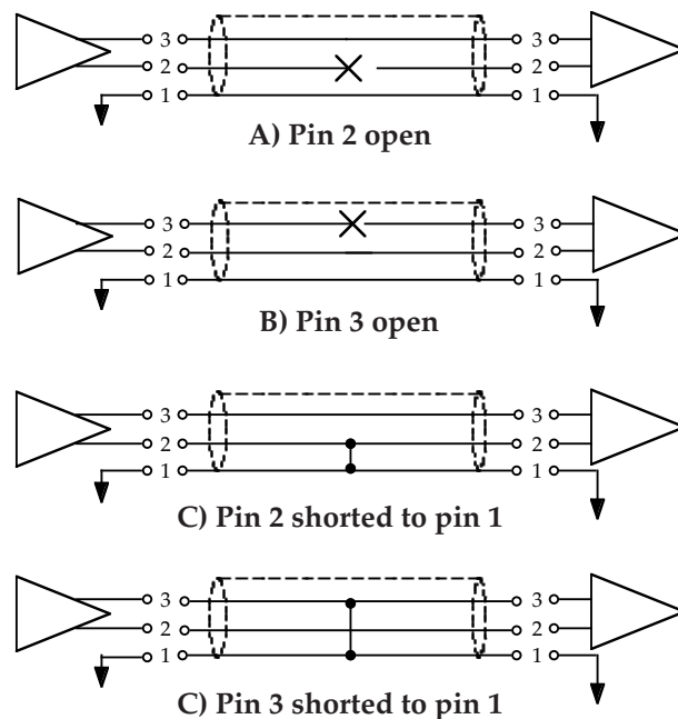
Fig 4.8f Unbalancing of a balanced line. Each of the above scenarios causes a 6 dB signal loss.
