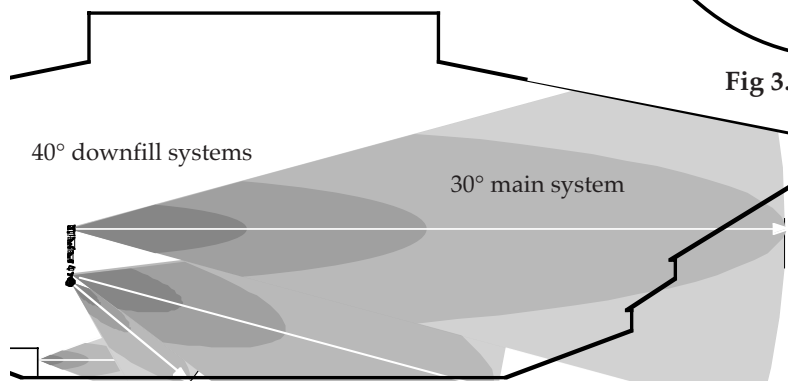
Fig 3.4r Section view of an example of an arena concert system.
