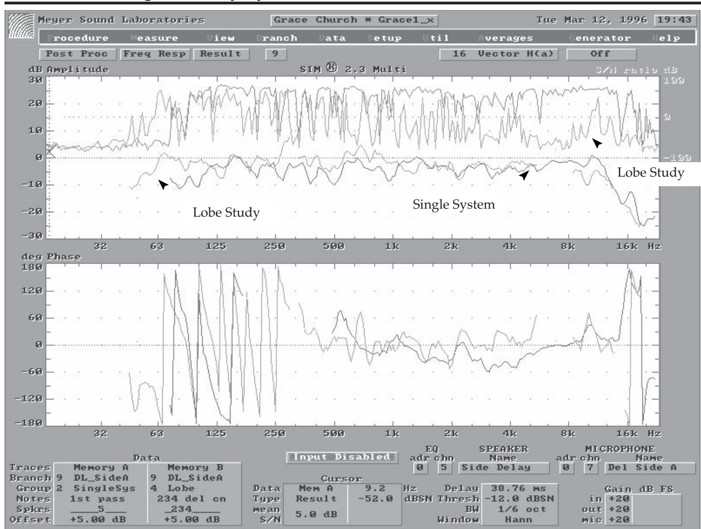
Fig 5.10m Evaluating the need for the delay speakers.
