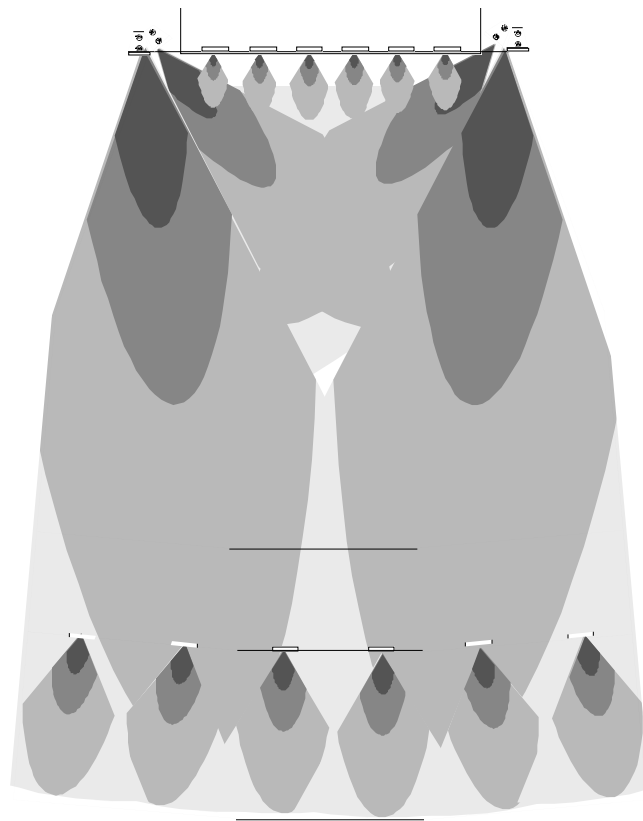
Fig 3.4m Plan view of an example of a musical theatre system.
